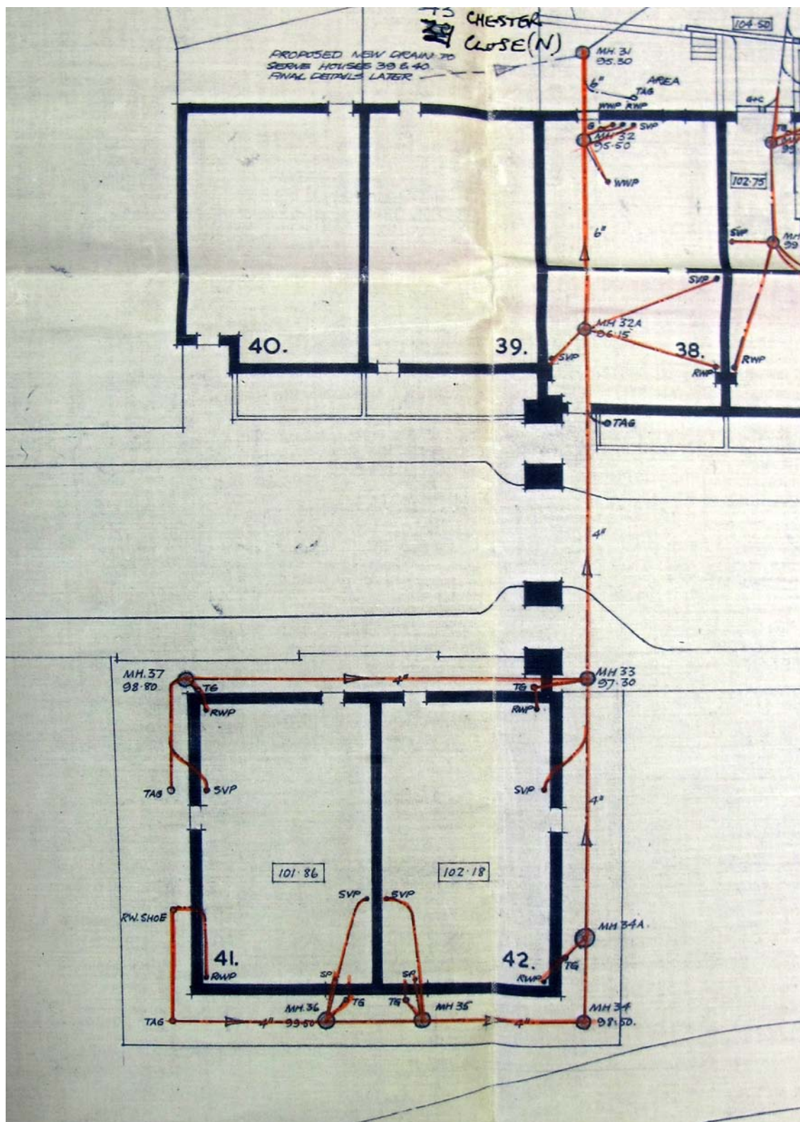
1961 41-42 Chester Terrace Drainage Plan
