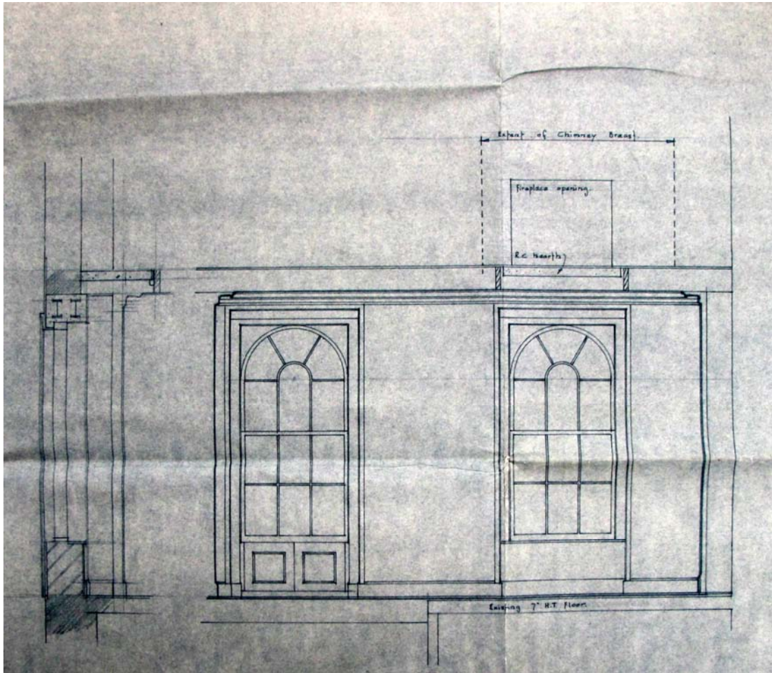
1962 42 Chester Terrace Proposed New Window for Dining Room Elevation
