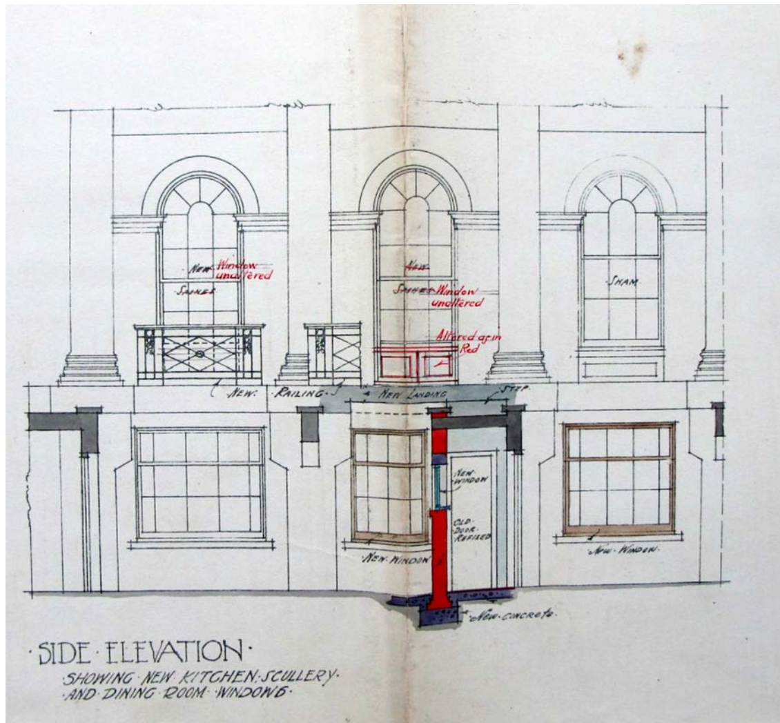
1925 41 CT Side Elevation Proposed
