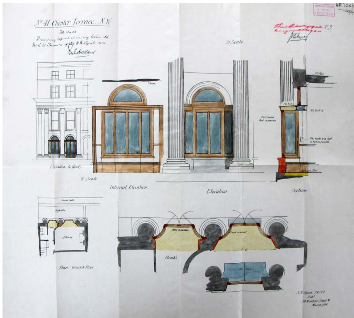
1914 41 CT Alterations to Windows
