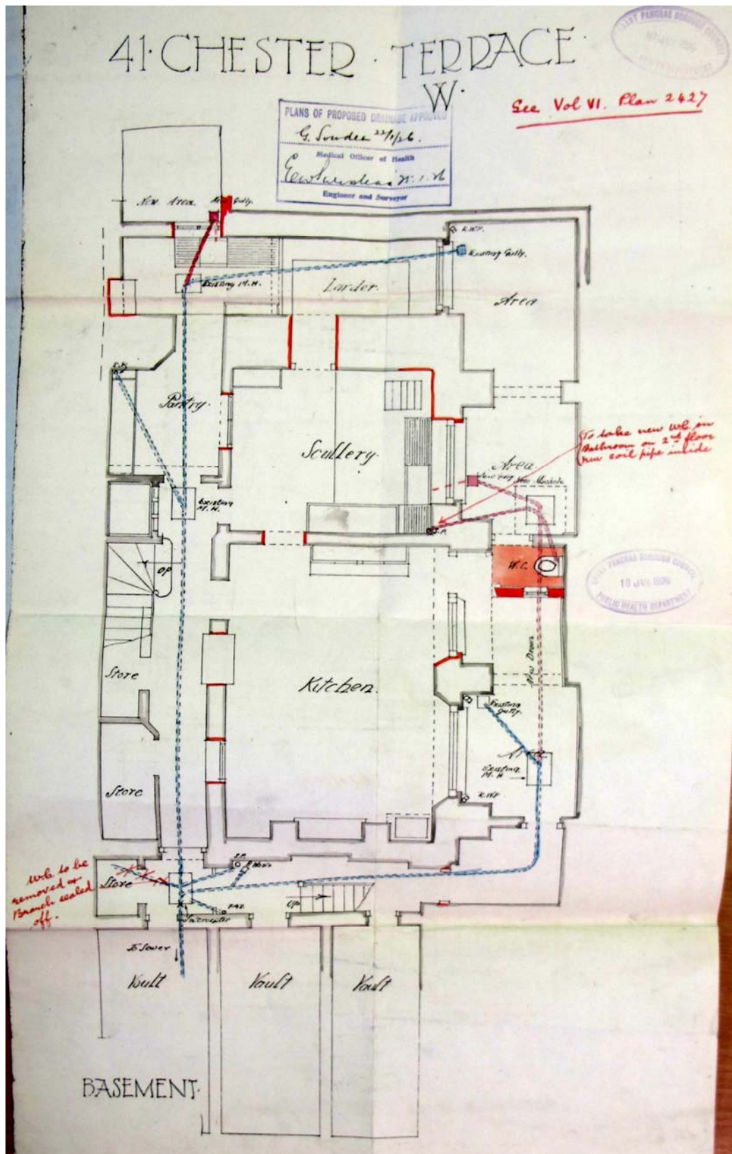
1926 41 CT Drainage Plan
