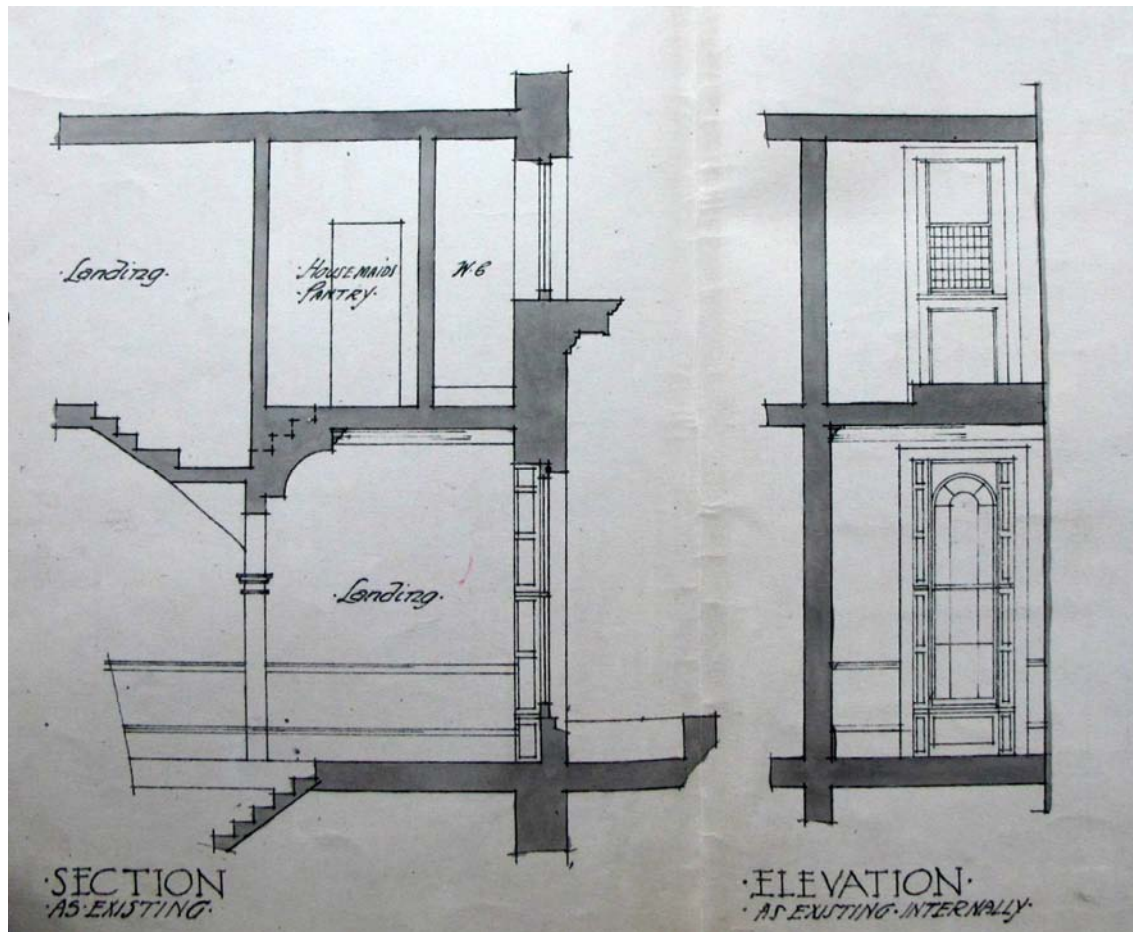
1925 41 CT Section and Elevation Existing
