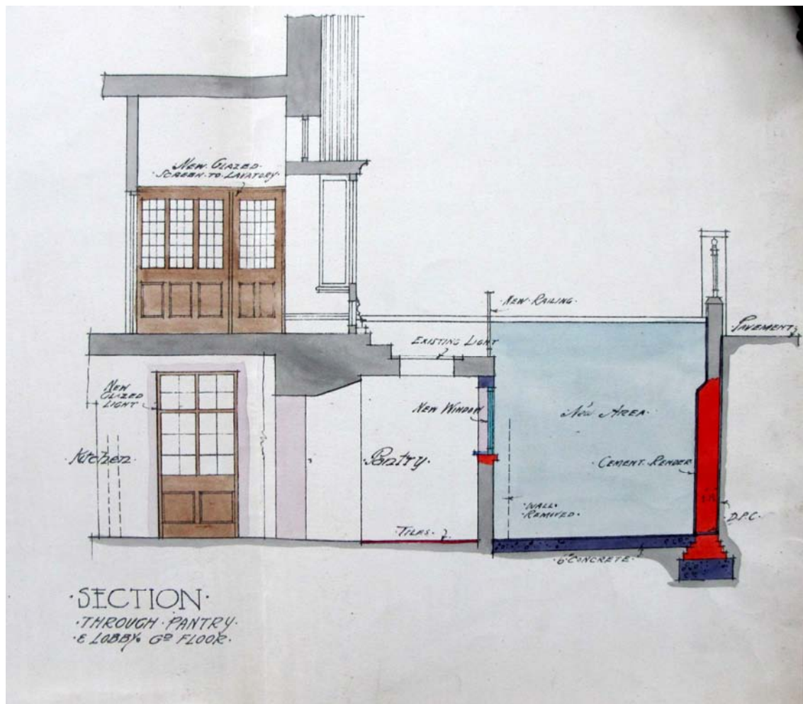
1925 41 CT Section trough pantry Proposed
