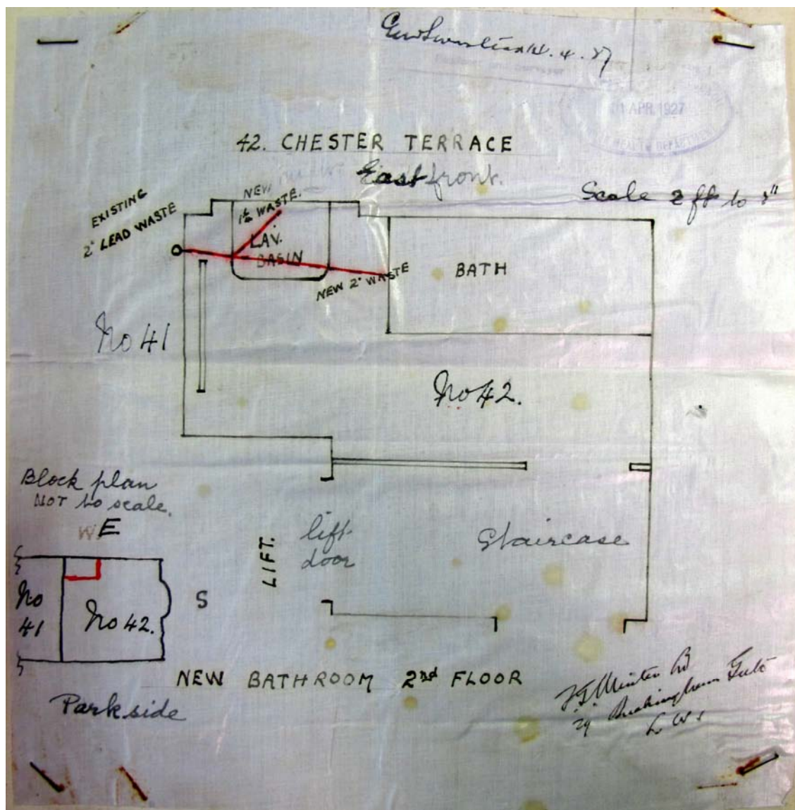
1927 42 CT Drainage Plan
