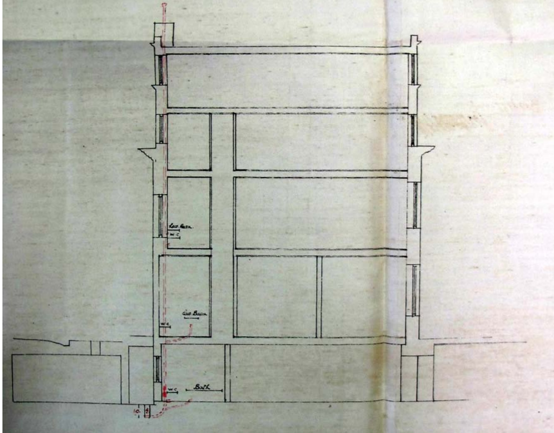
1920 42 CT Section
