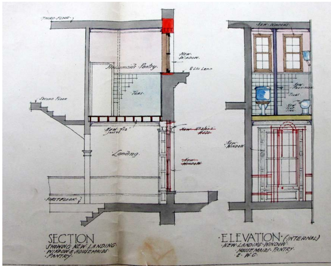
1925 41 CT Section and Elevation Proposed
