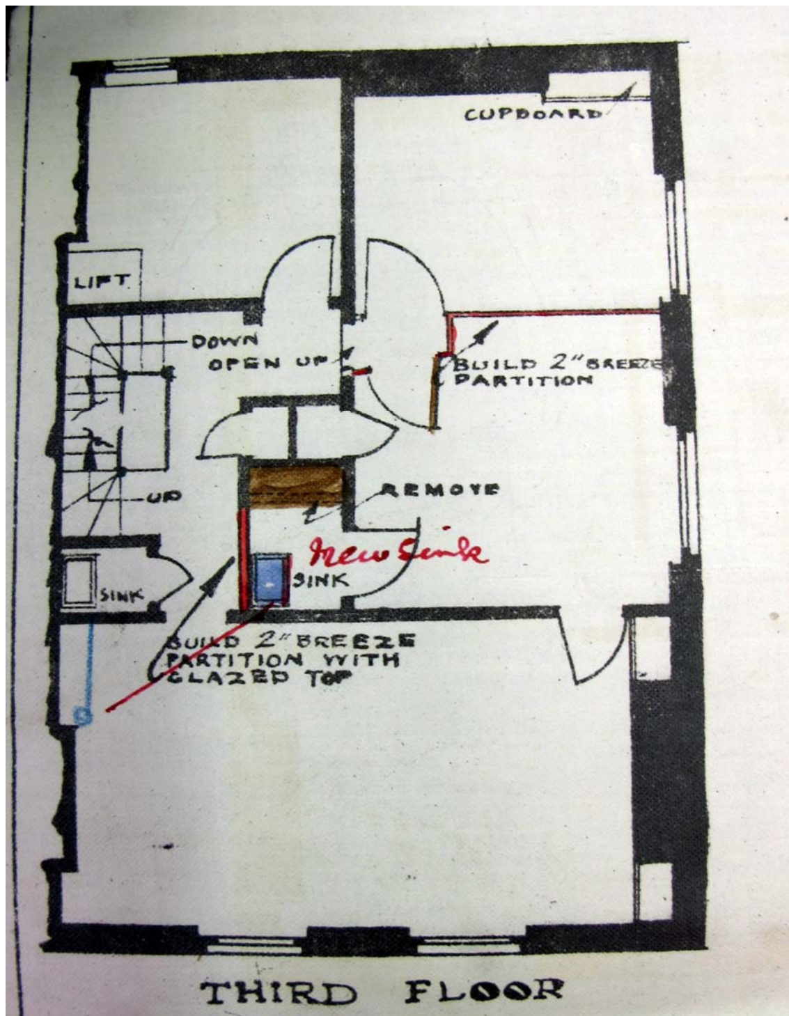
1932 42 CT Third Drainage Plan
