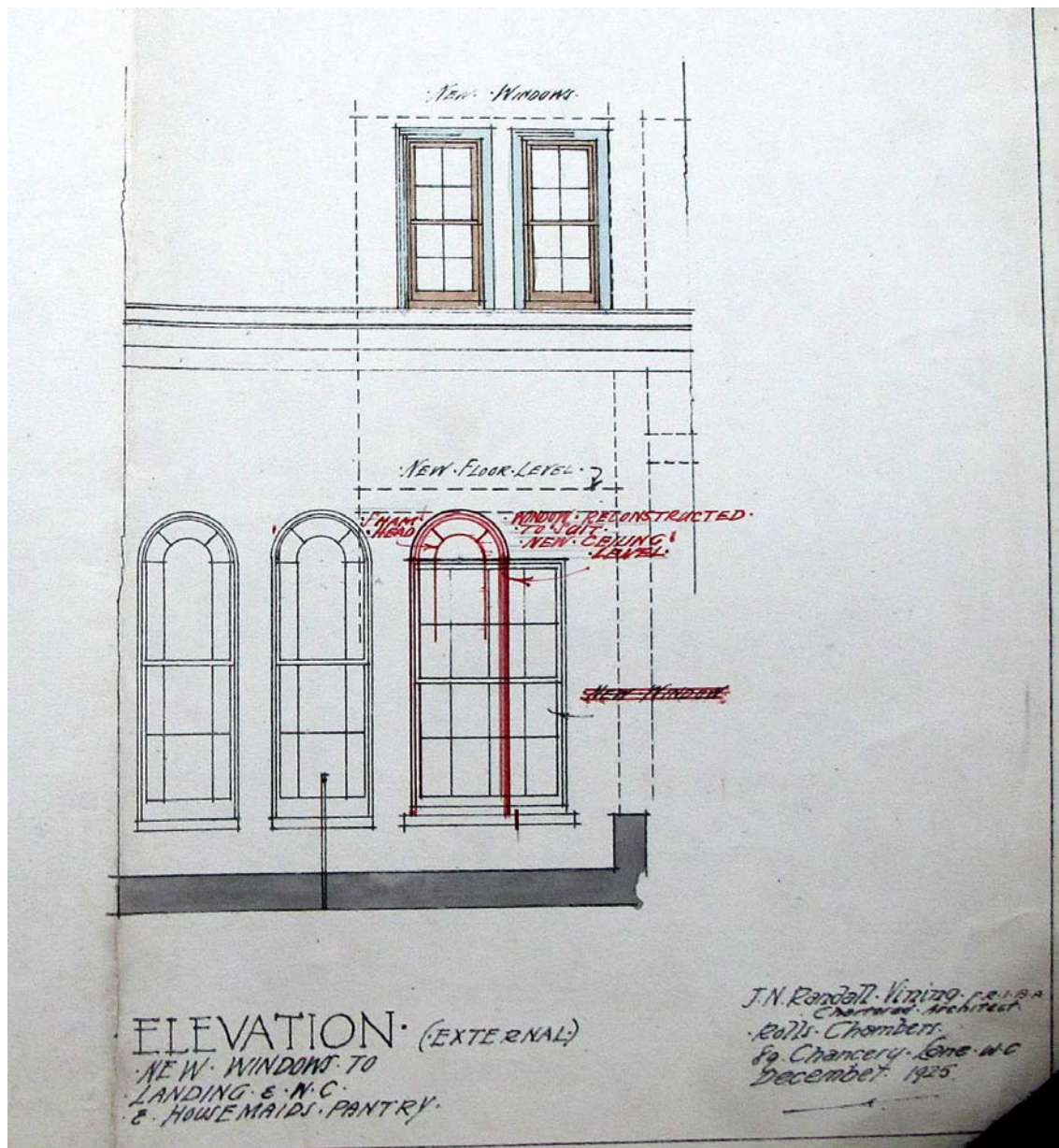
1925 41 CT Elevation Proposed
