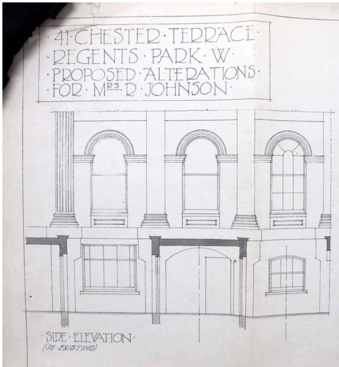
1925 41 CT Side Elevation Existing
