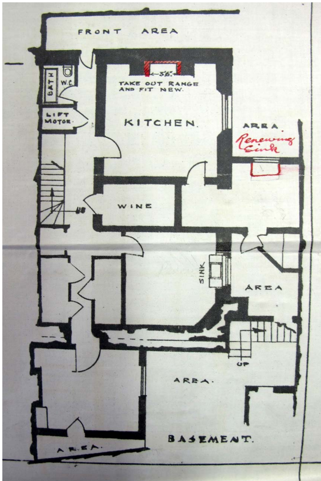
1932 42 CT Basement Drainage Plan
