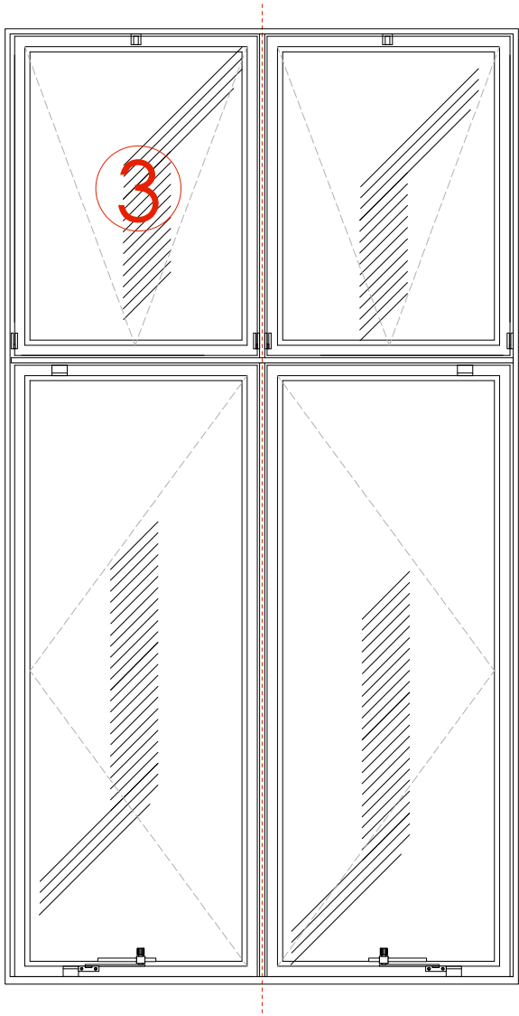
1 Type 3 window elevation (Lightwell 3) 1:10 @ A1
