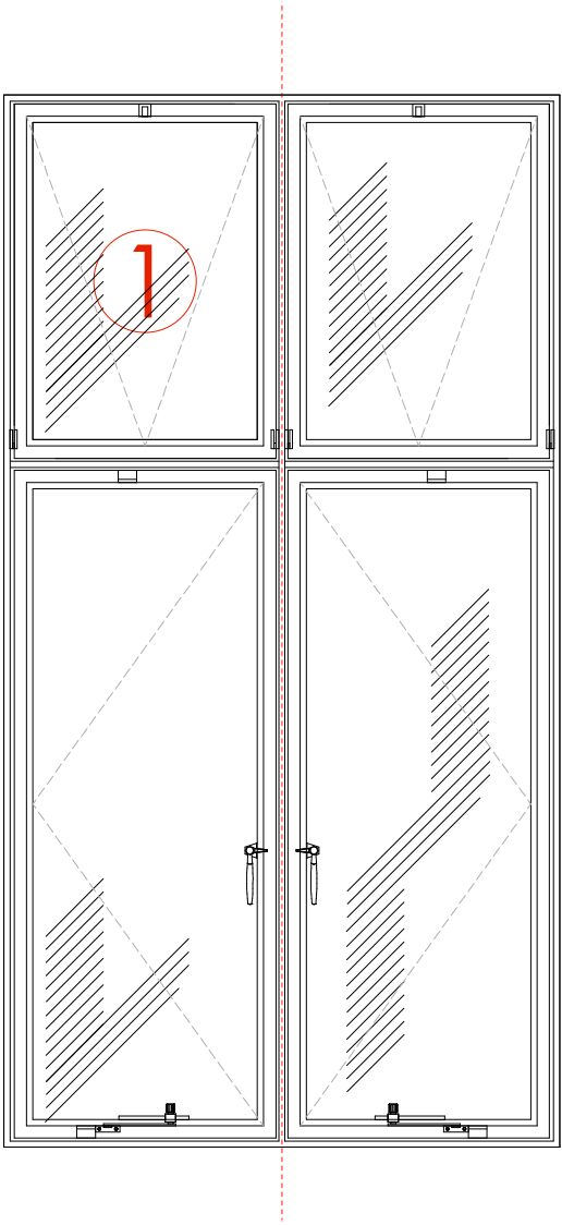
1 Type 1 window elevation (Lightwell 3) 1:10 @ A1
