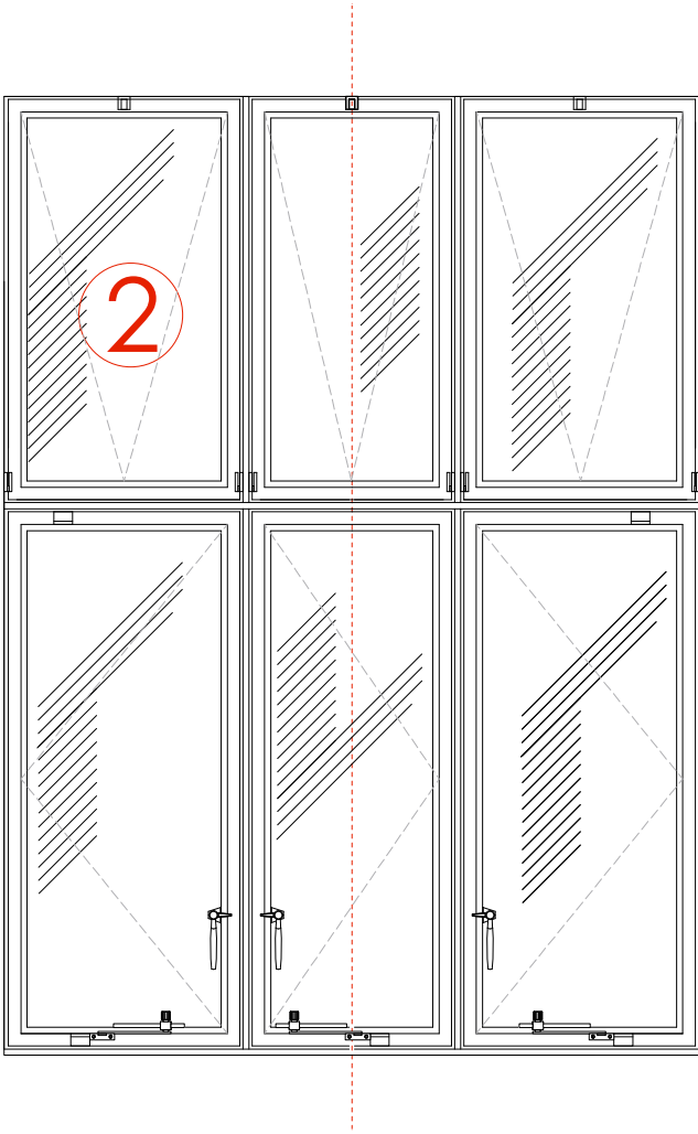
2 Type 2 window elevation (Lightwell 3) 1:10 @ A1
