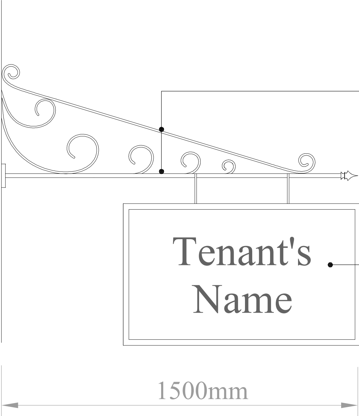
Front and Side Elevation of Sign 1:10@A1 (1:20@A3)
