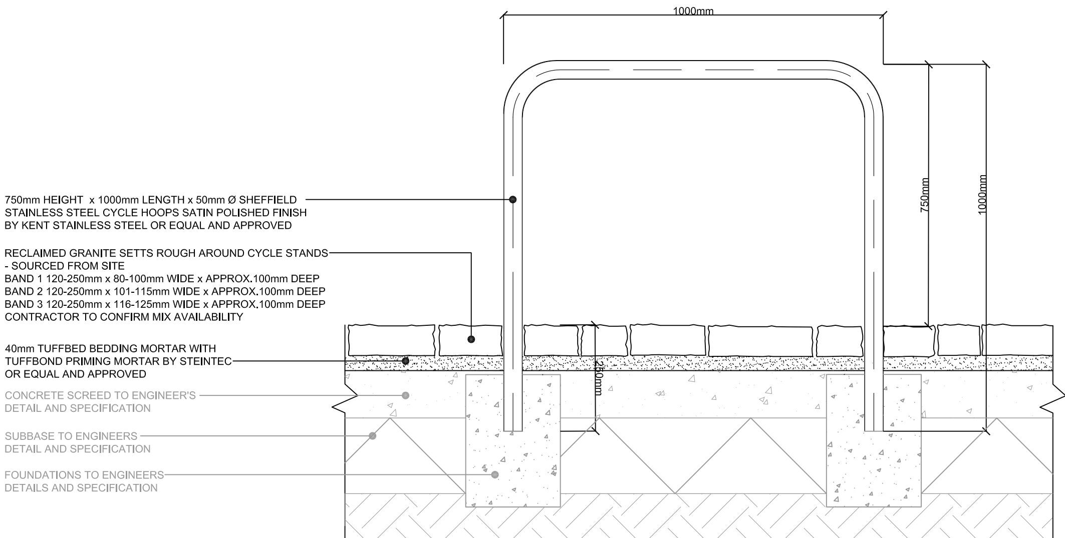
DETAIL 4.04 CYCLE STAND INTERFACE WITH GRANITE SETTS SCALE 1:10
