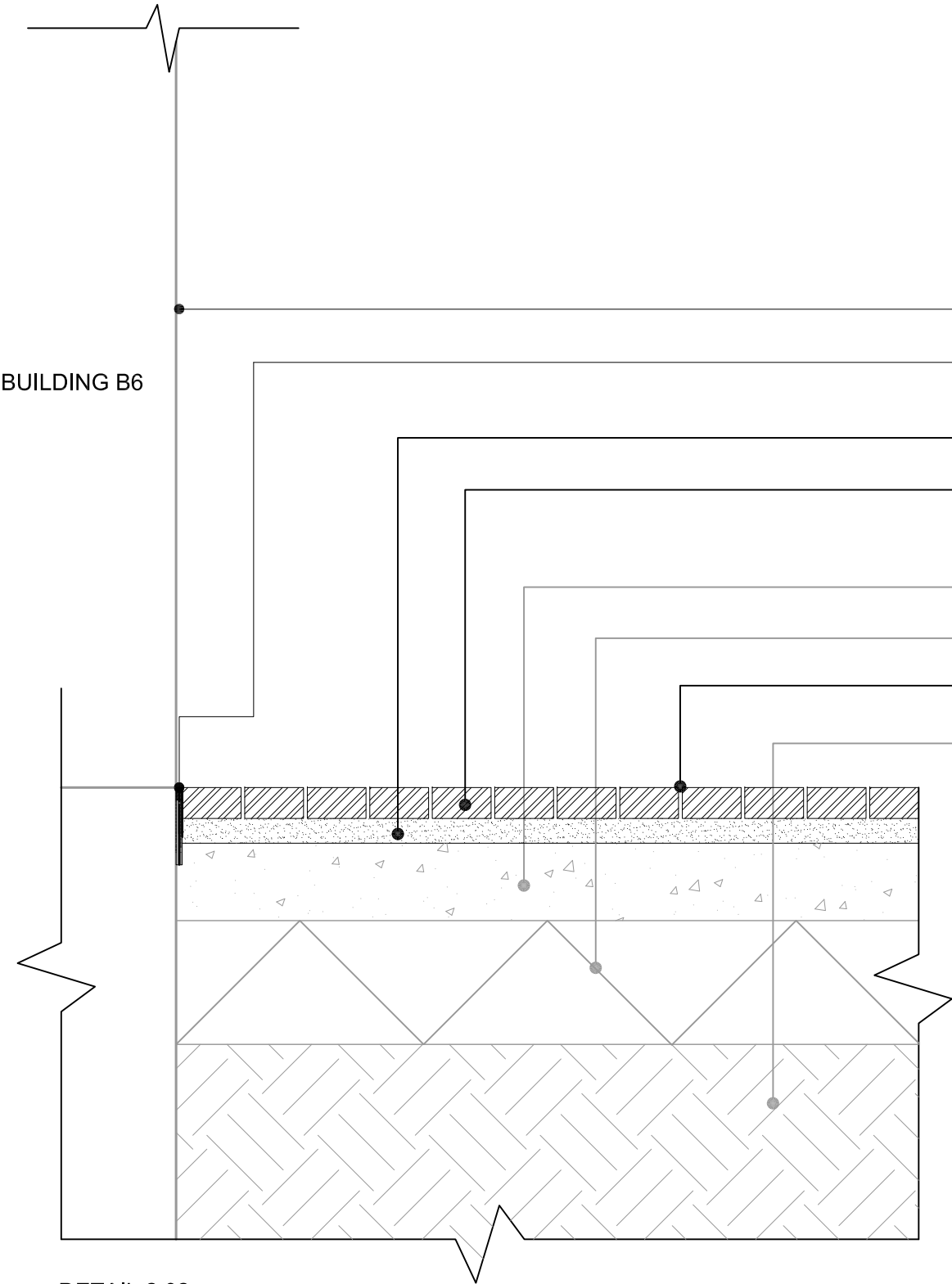
DETAIL 2.02 PAVING PATTERN 6 INTERFACE WITH BUILDING FACADE SCALE 1:10
