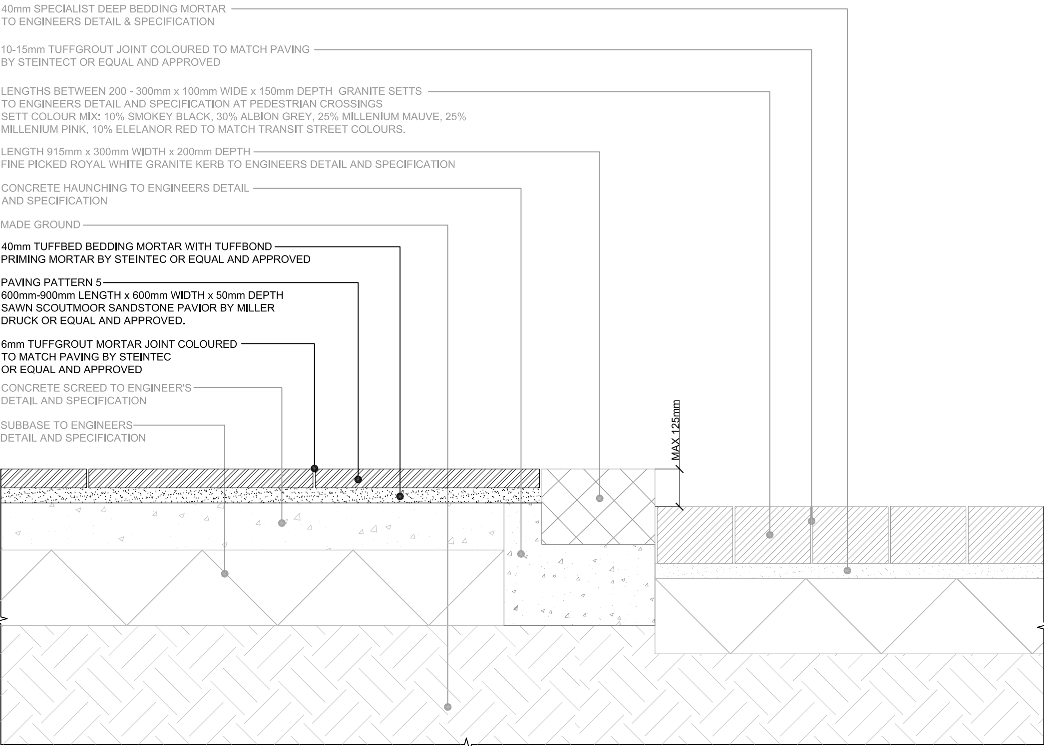
DETAIL 1.03 PAVING INTERFACE WITH GRANITE KERB SCALE 1:10
