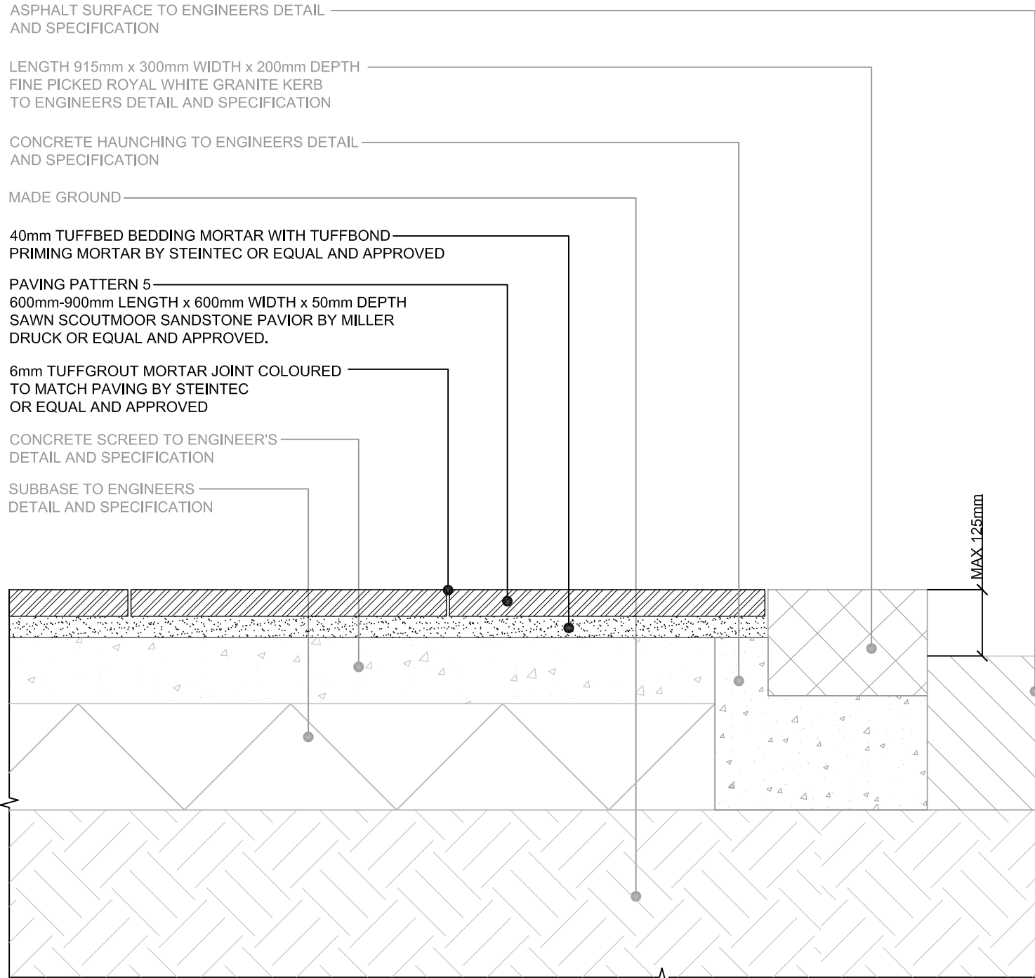
DETAIL 1.02 PAVING INTERFACE WITH GRANITE KERB SCALE 1:10
