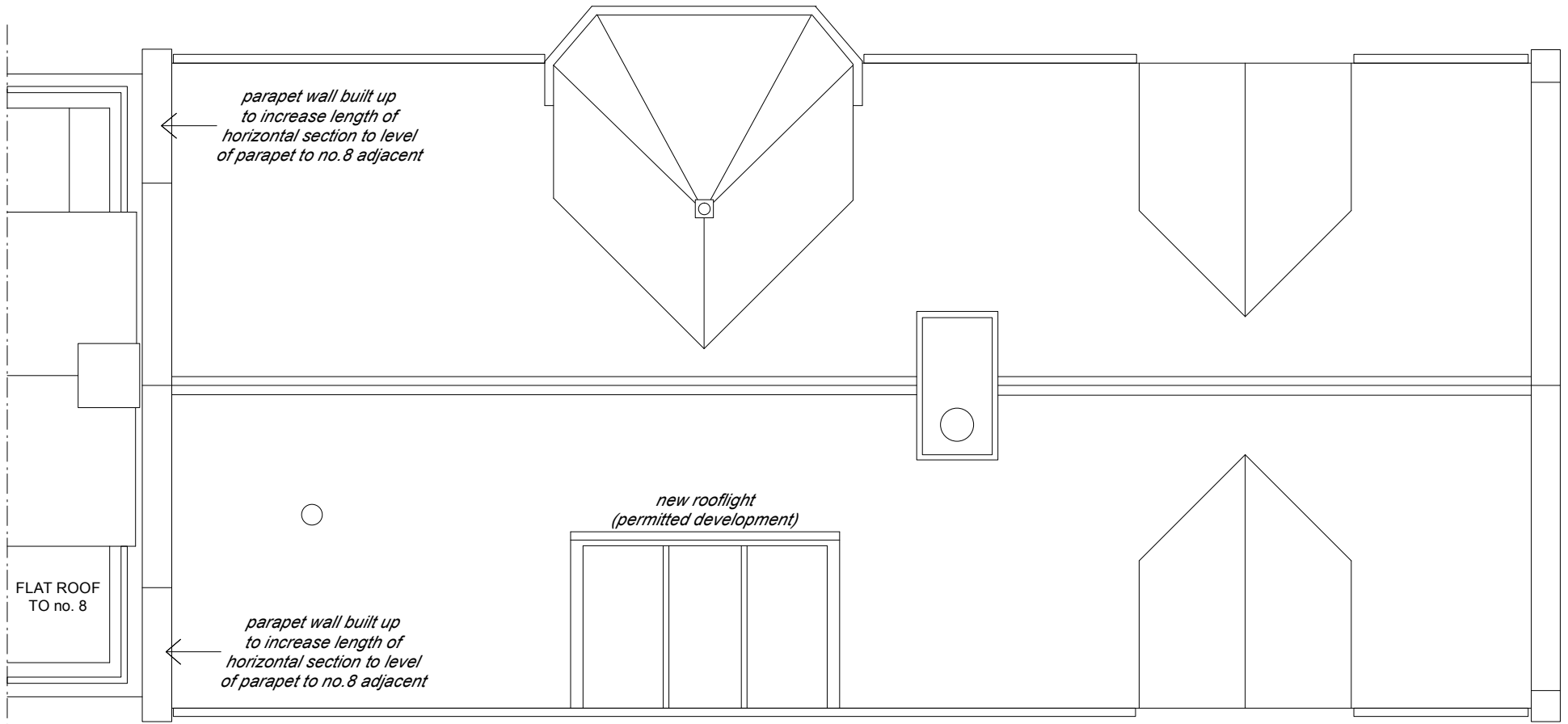
ROOF PLAN
