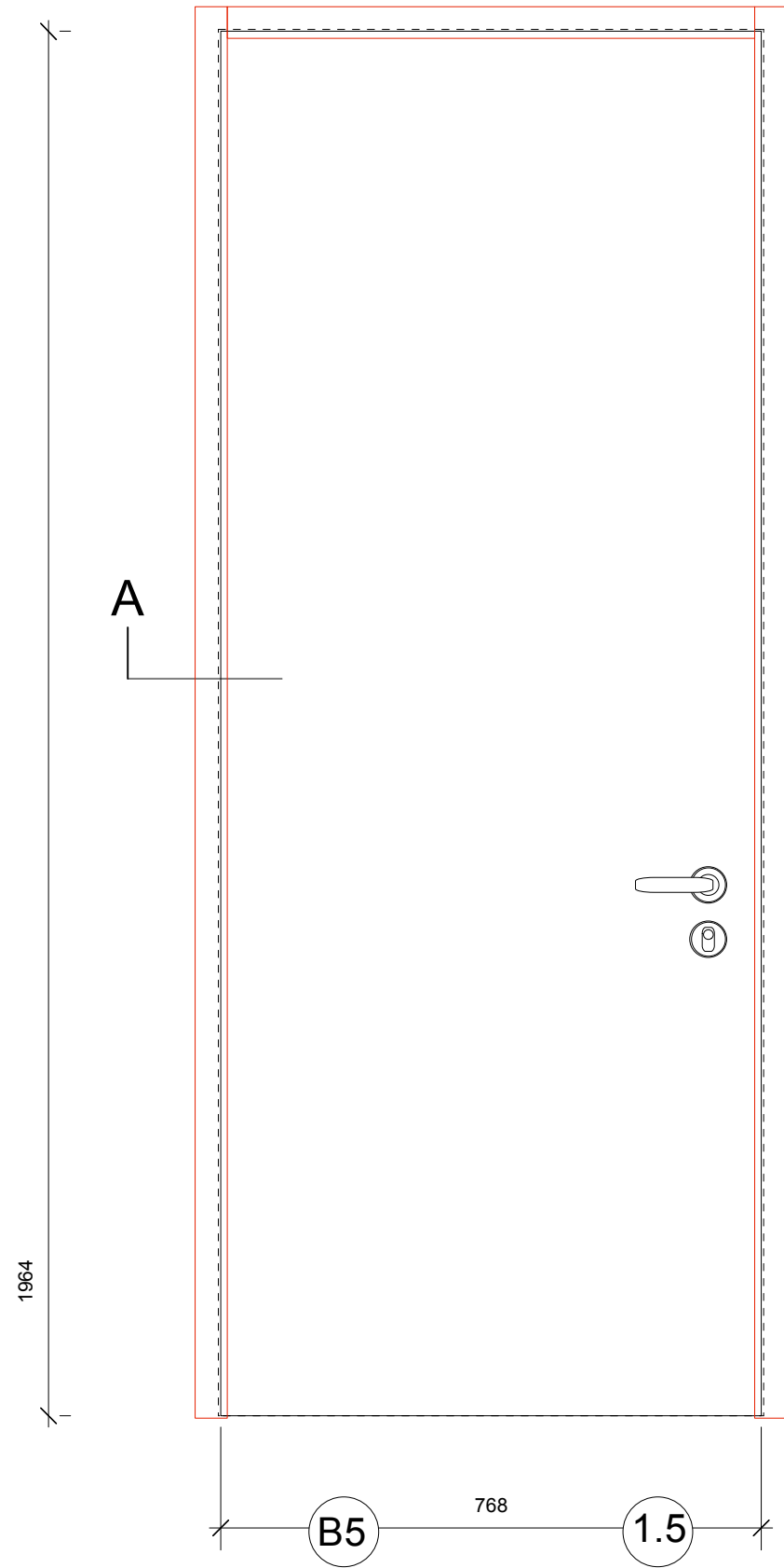
CORRIDOR ELEVATION
