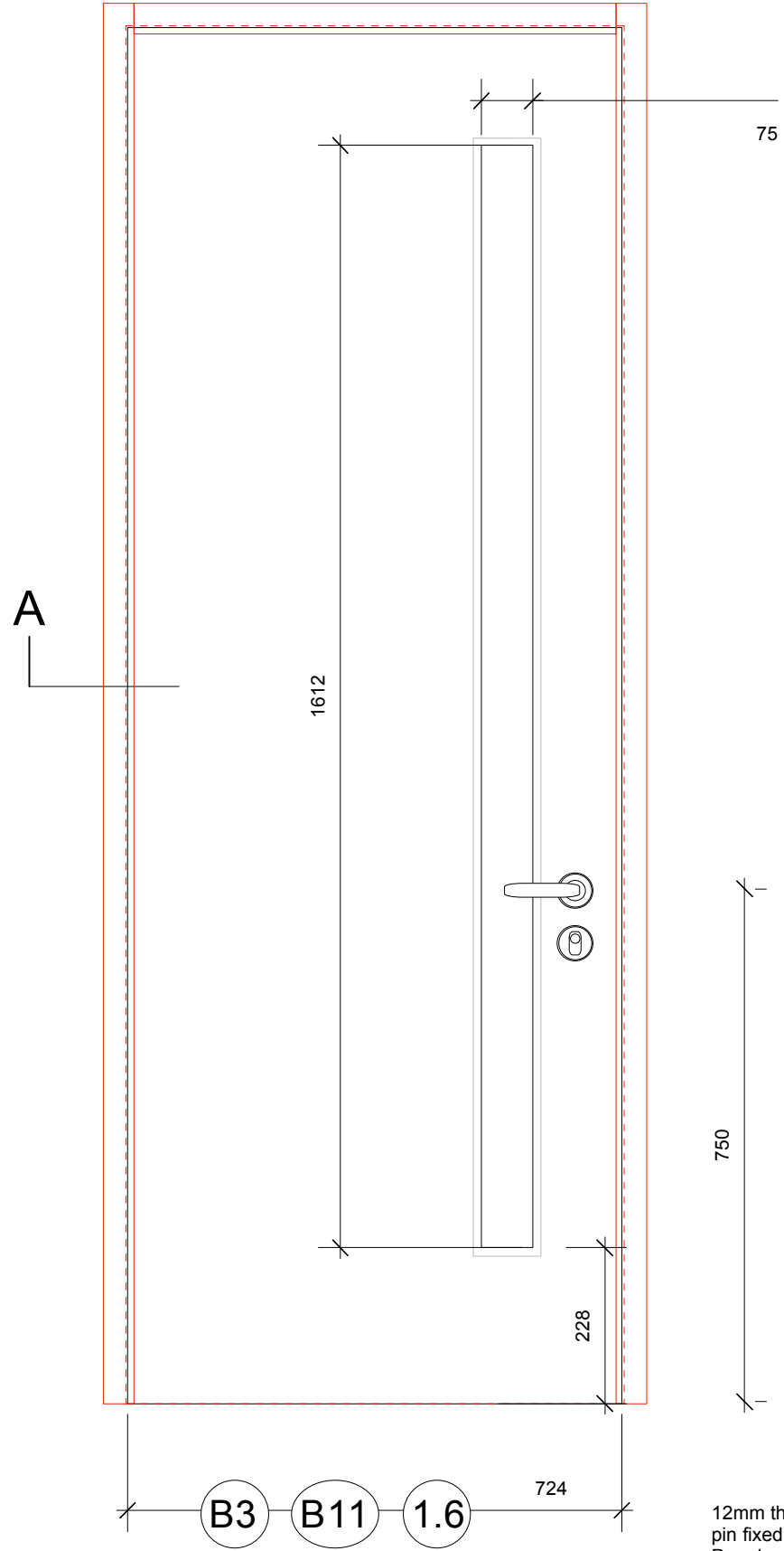
CORRIDOR ELEVATION
