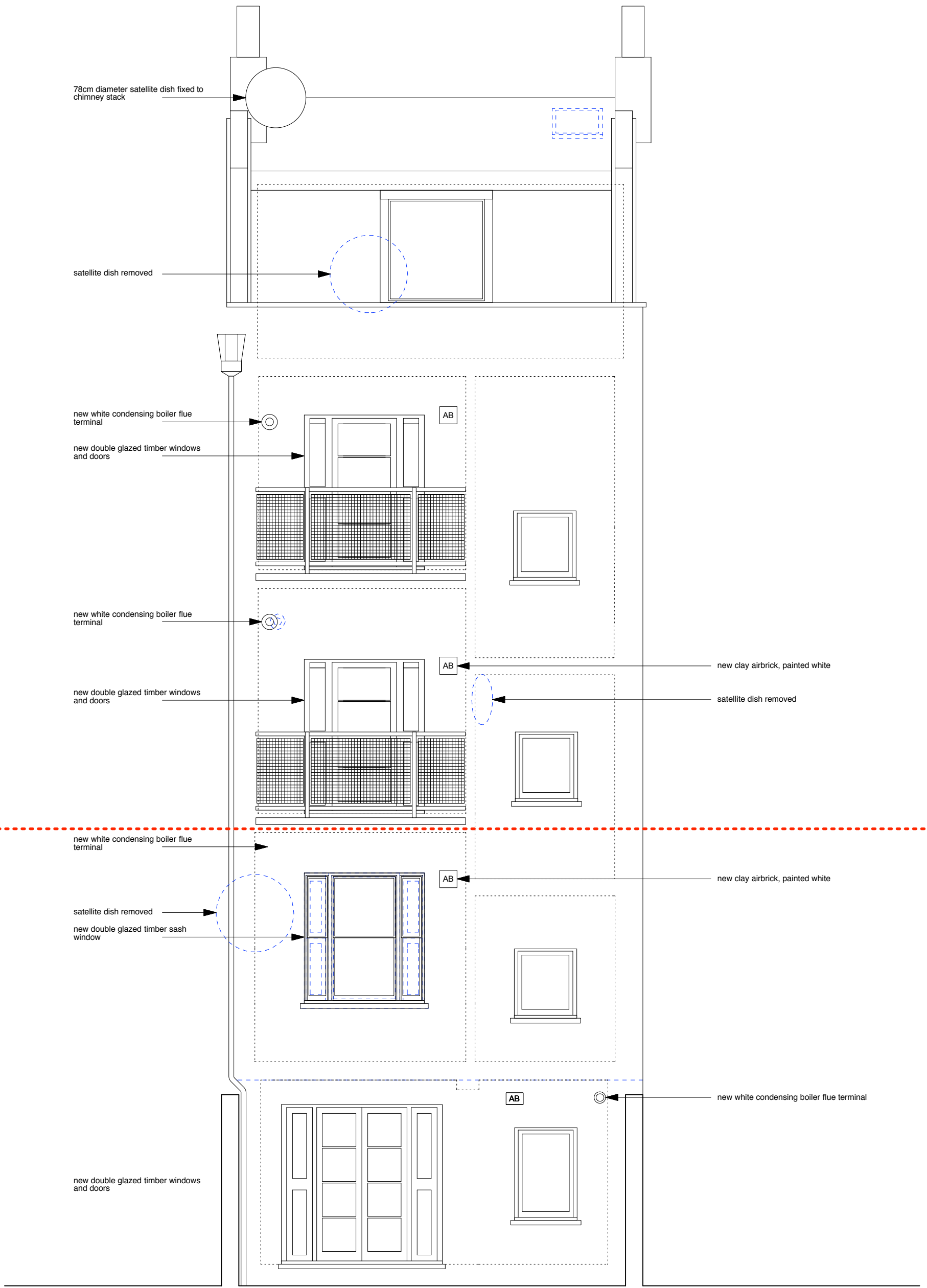
REAR ELEVATION
