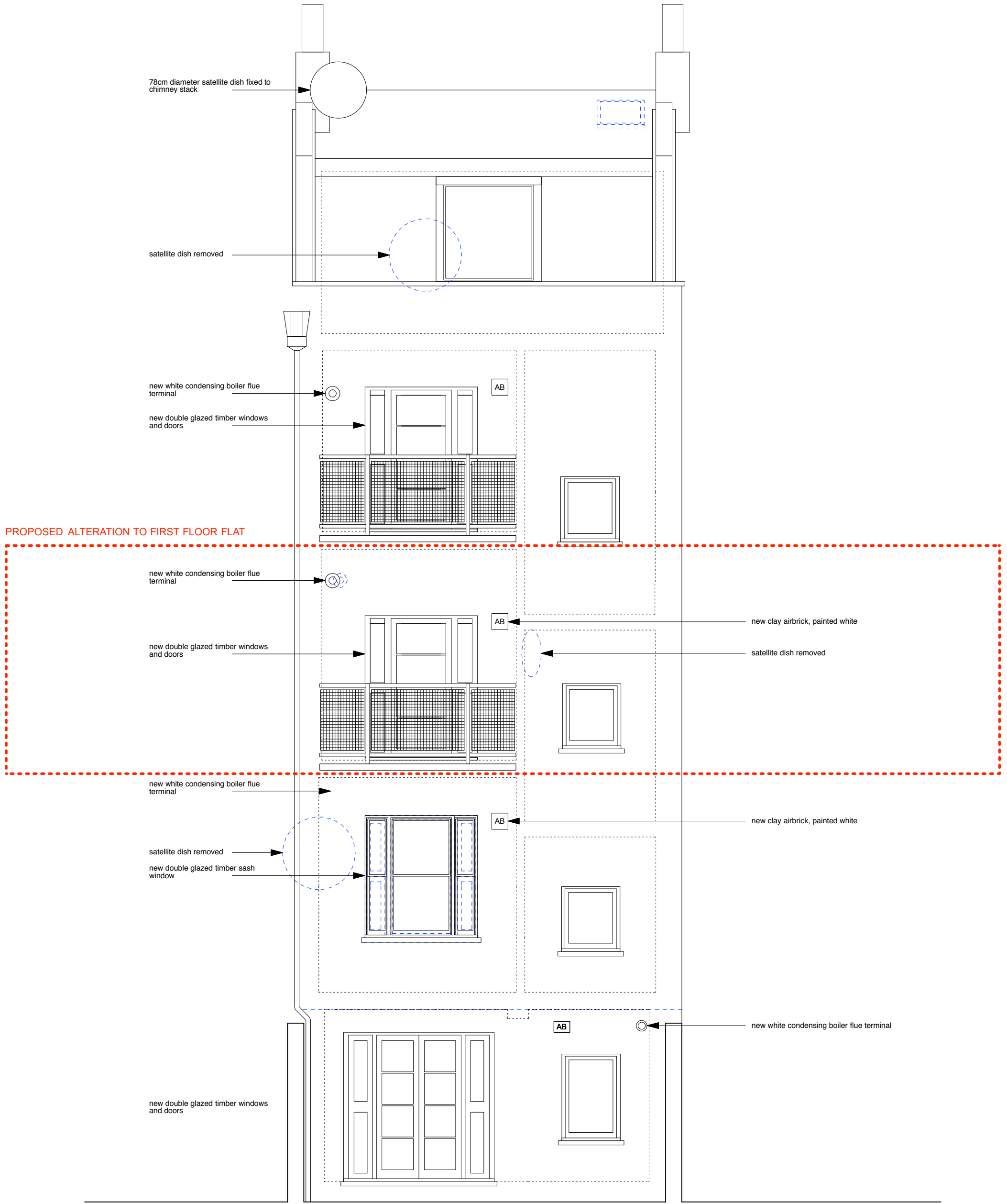
REAR ELEVATION
