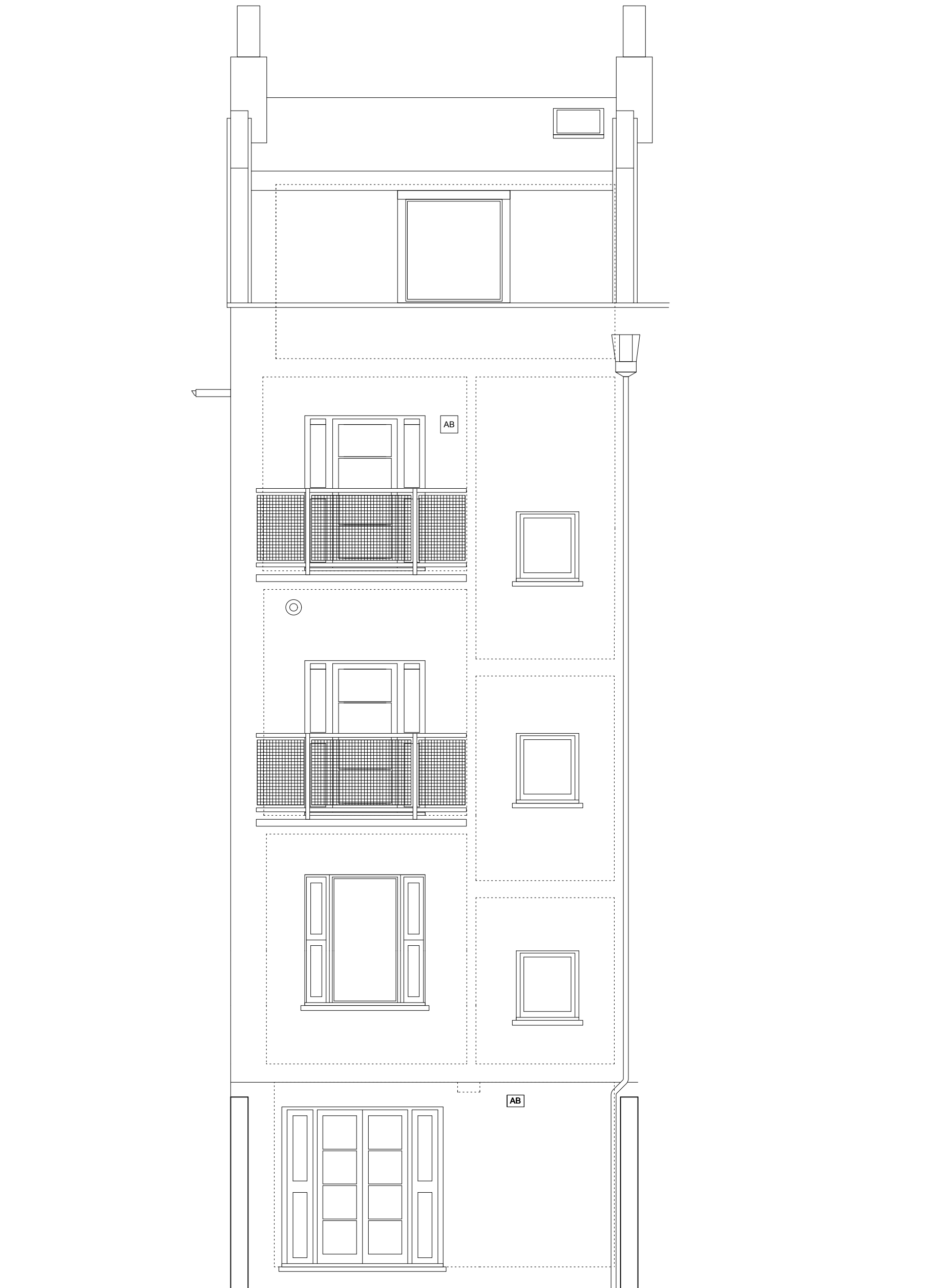
REAR ELEVATION
