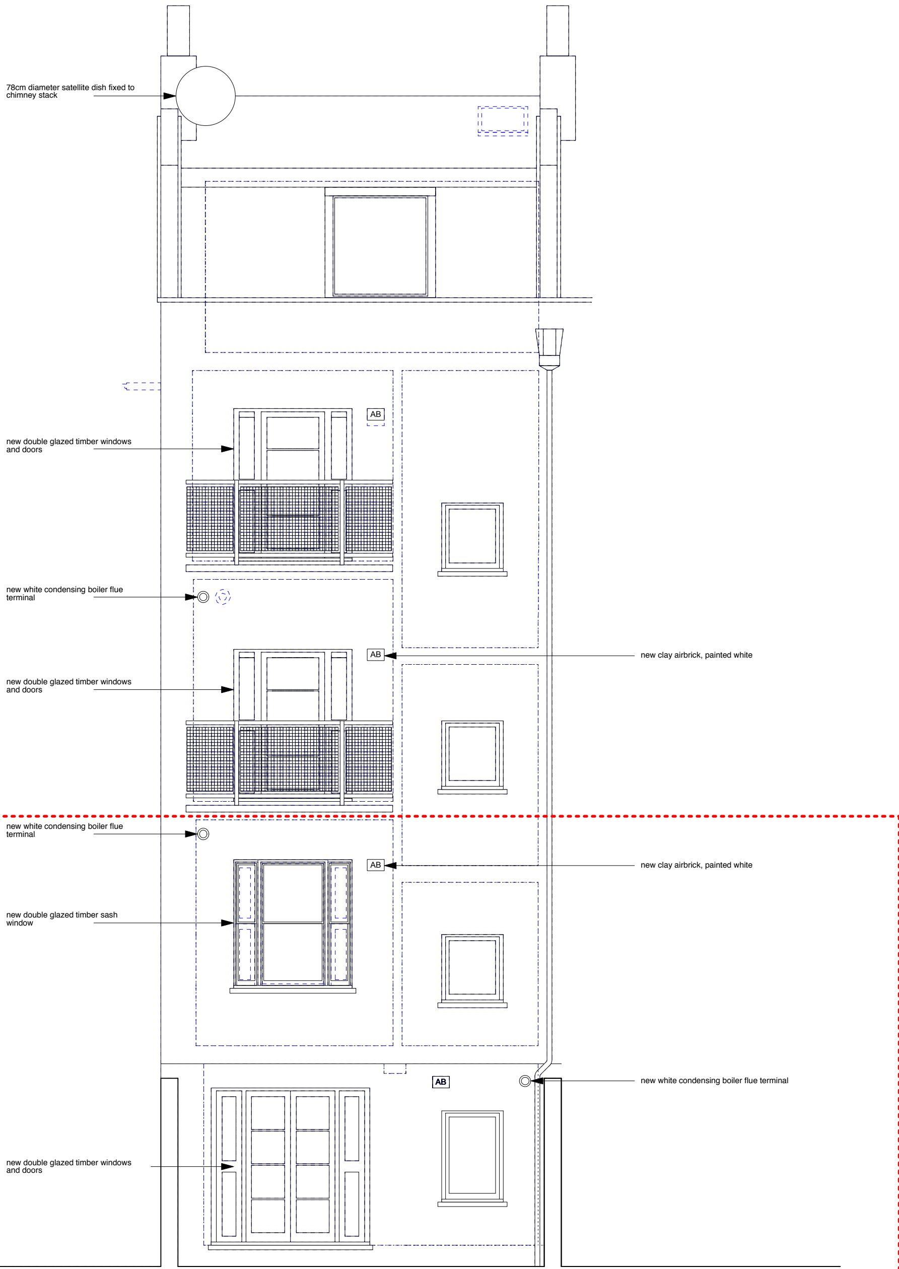
REAR ELEVATION
