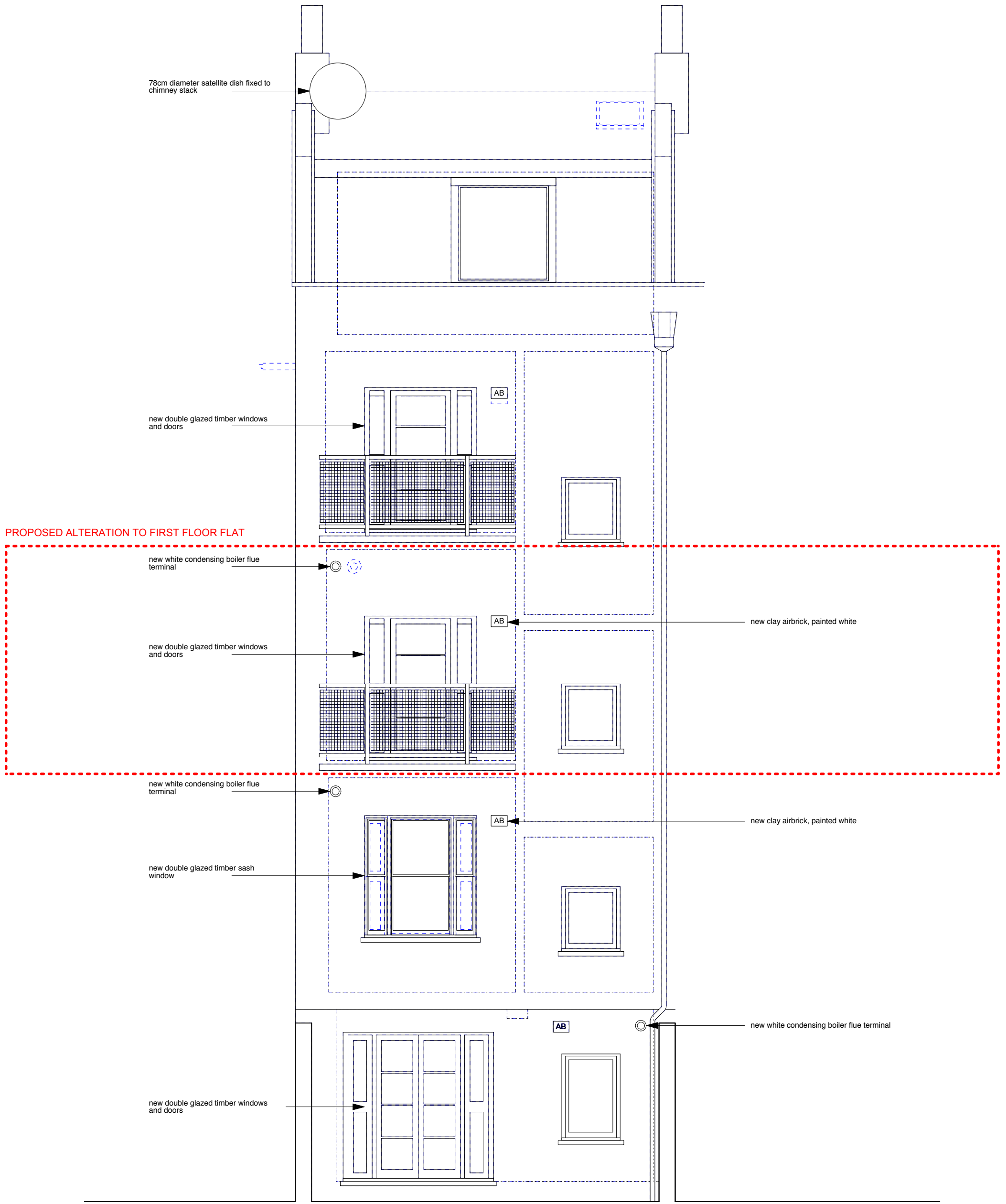
REAR ELEVATION
