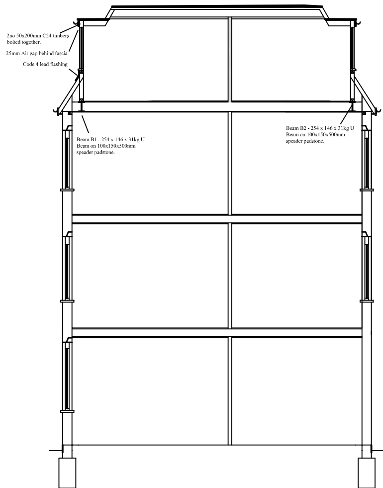
Proposed Section A-A
