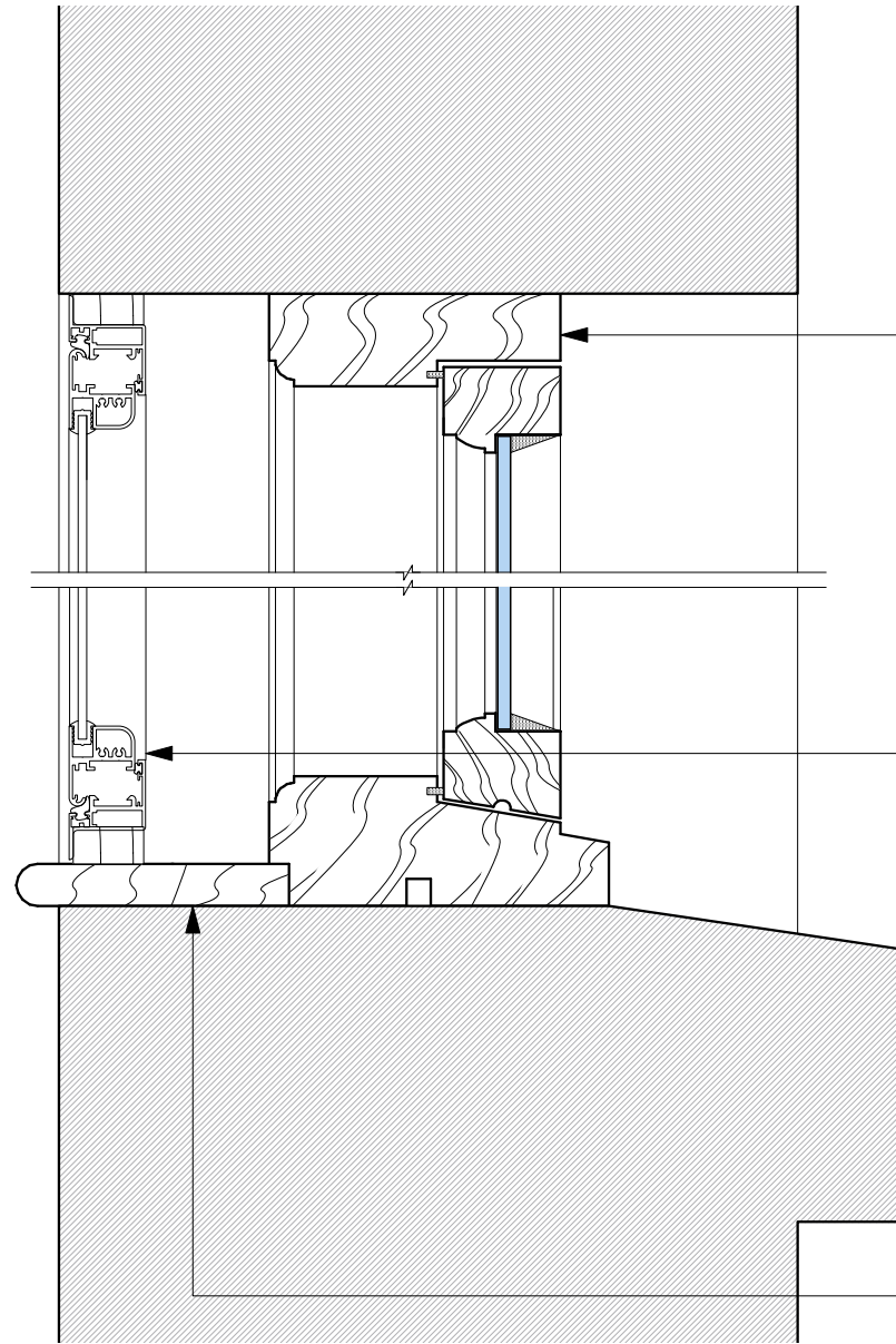
2 - Typical Cill Detail 1:2 @ A1, 1:4 @ A3
