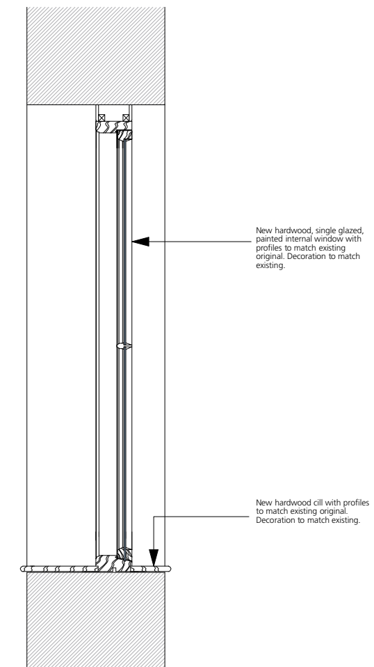
3 - Proposed Section 1:10 @ A1, 1:20 @ A3
