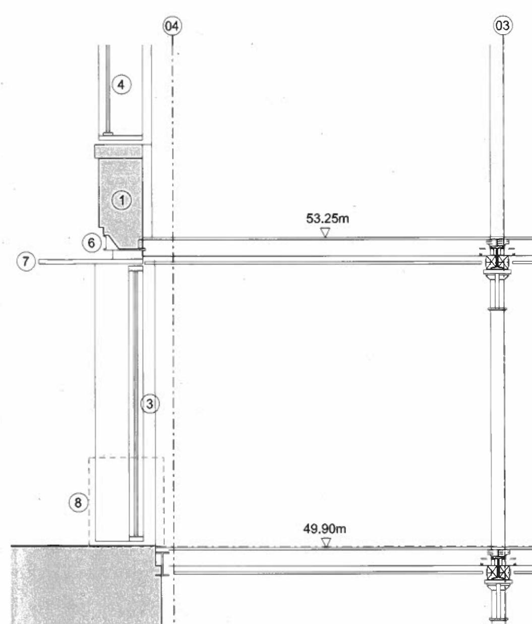
SECTION
