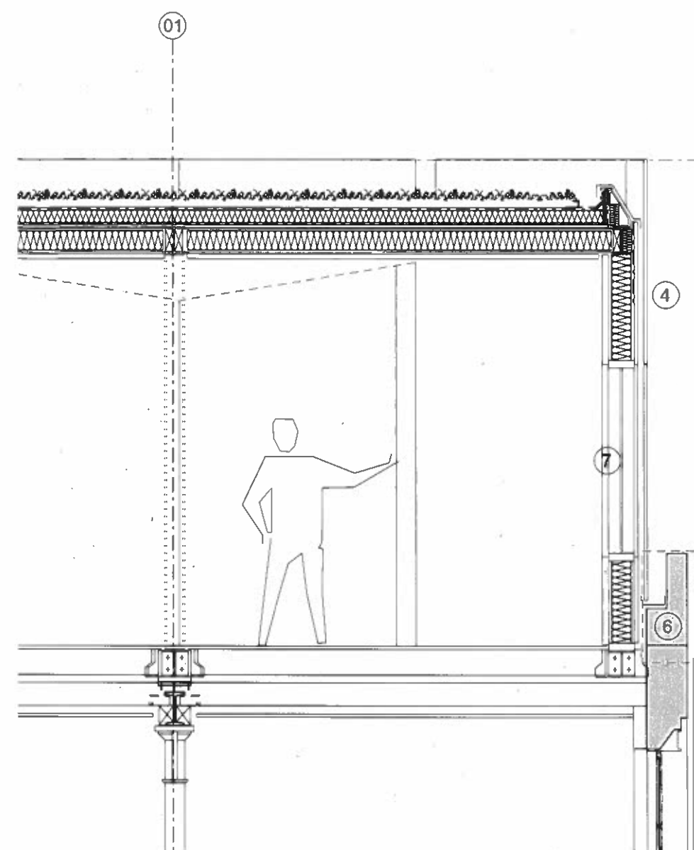
SECTION
