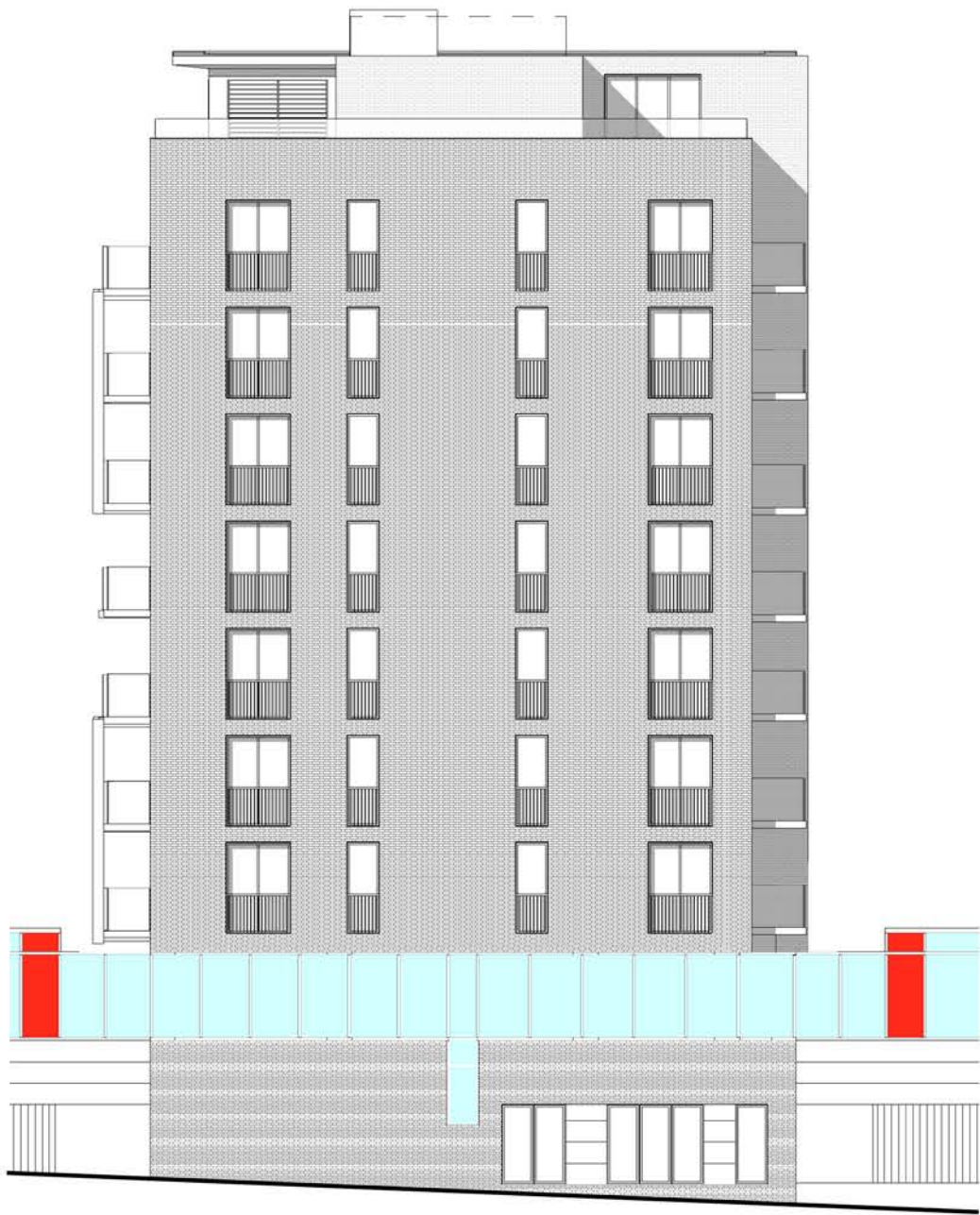
NORTH ELEVATION
