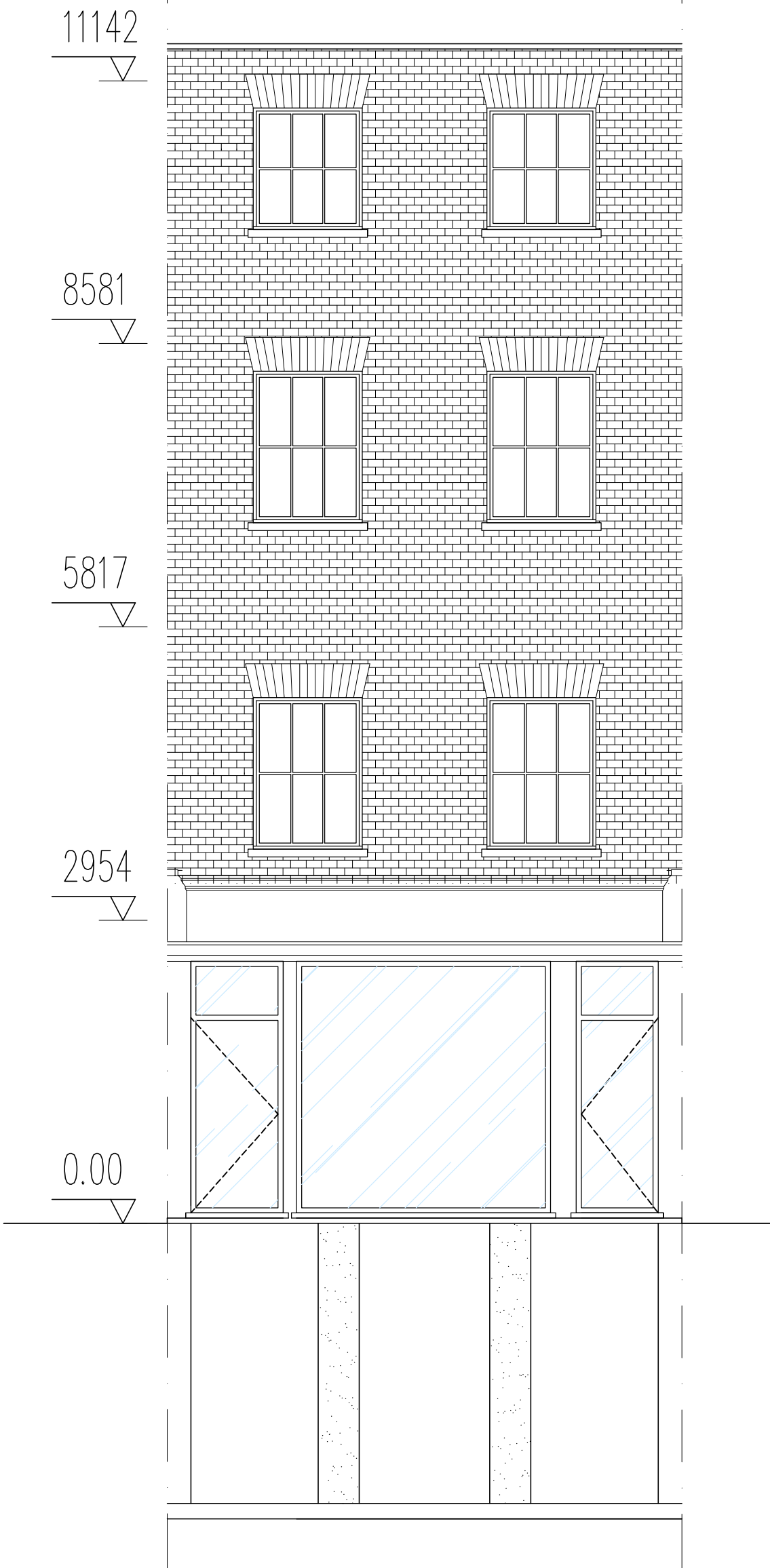
Front Elevation as Proposed Showing Lightwell
