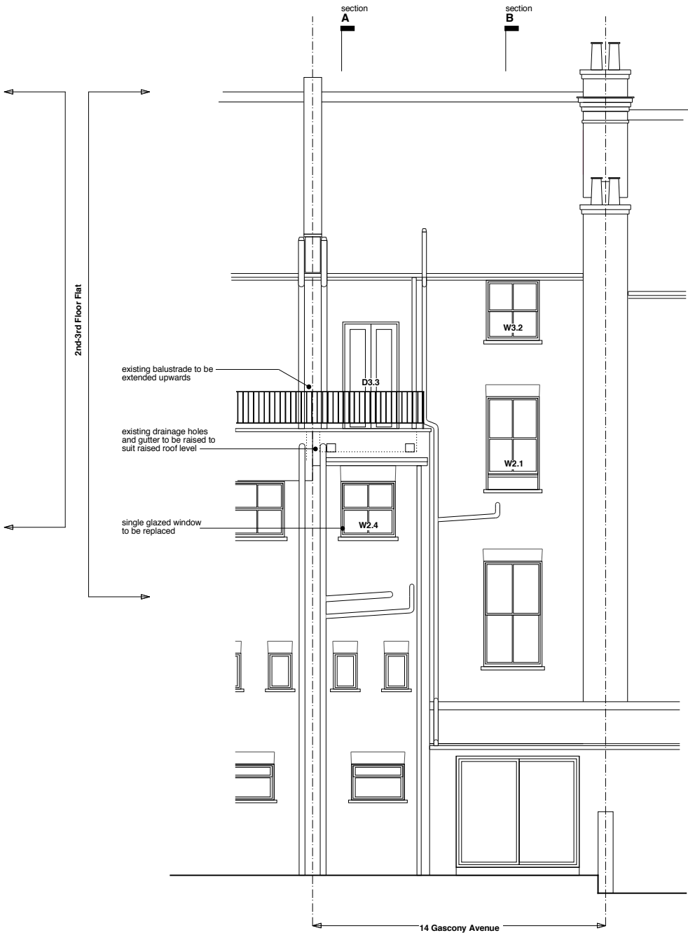
Rear Elevation
