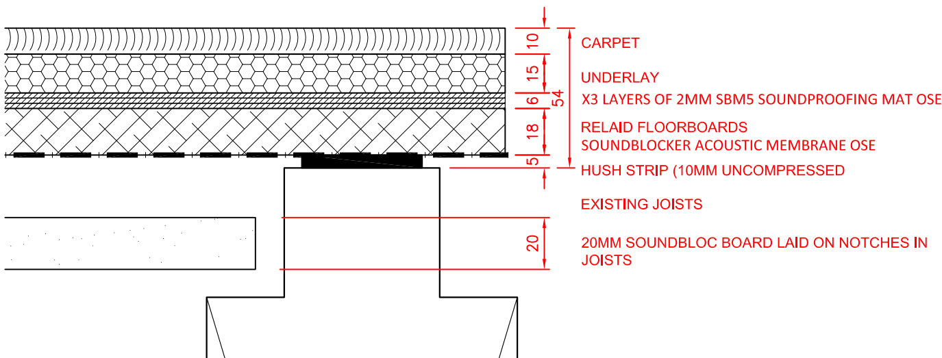
STANDARD CARPET DETAIL 1:2
