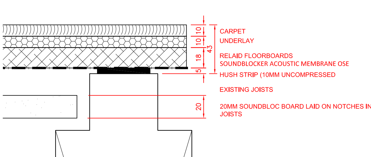
CARPET DETAIL HALL 1:2
