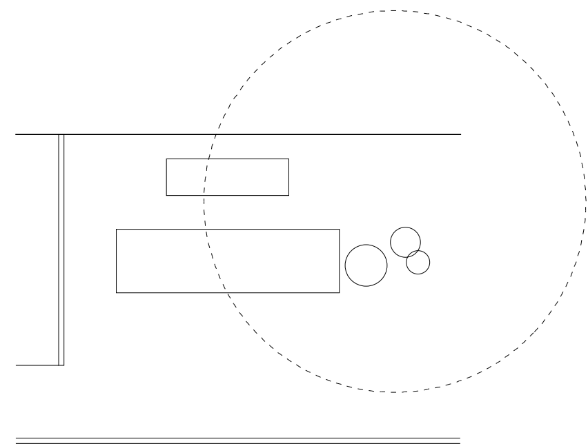
PLAN AS PROPOSED
