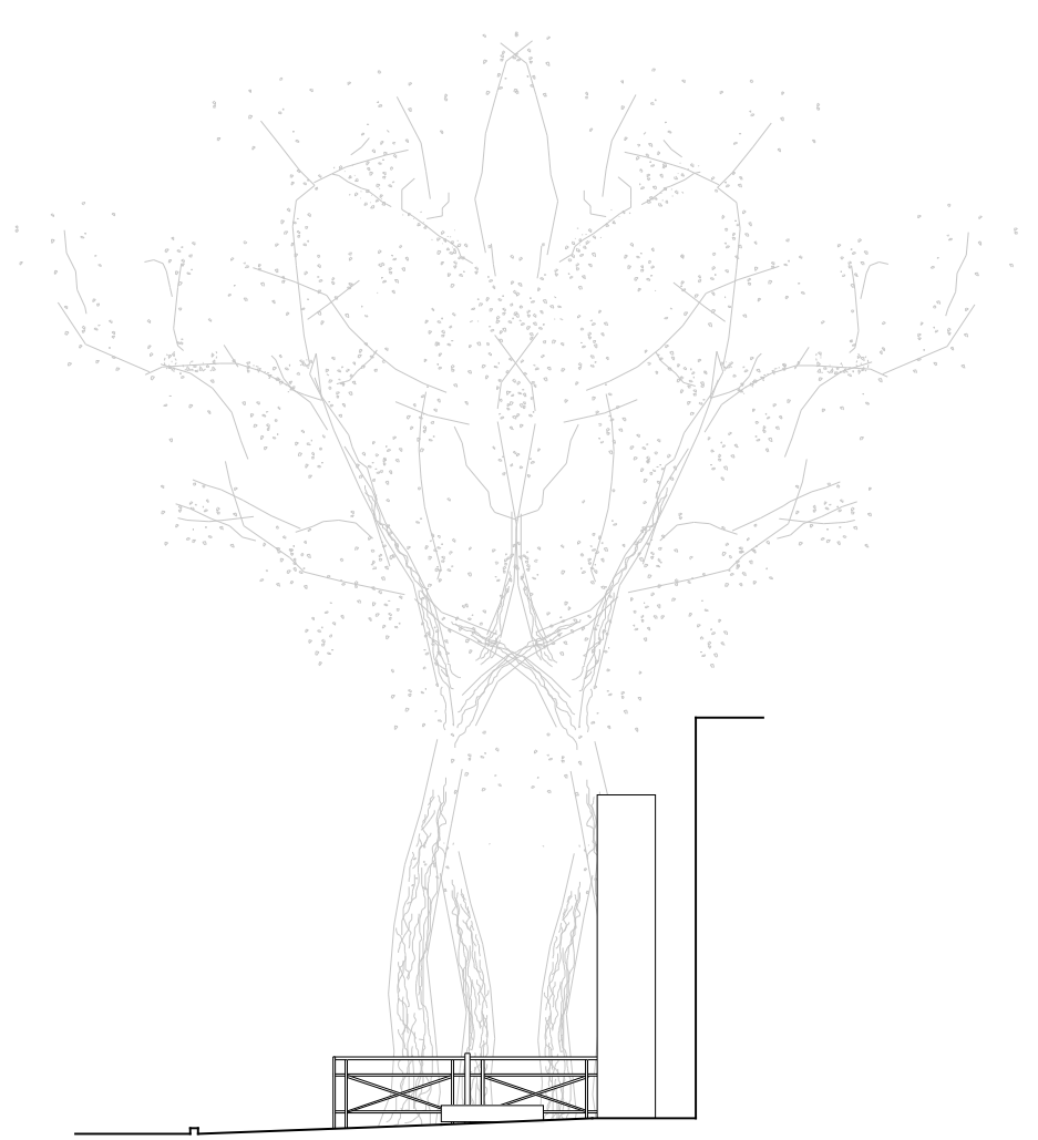
EAST ELEVATION AS PROPOSED
