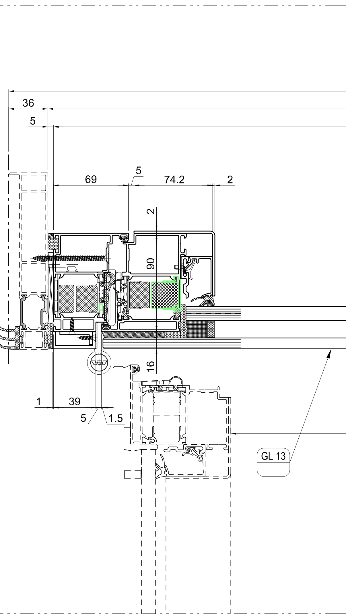
10 HORIZONTAL SECTION Door type 15 Single Scale: 1:2
