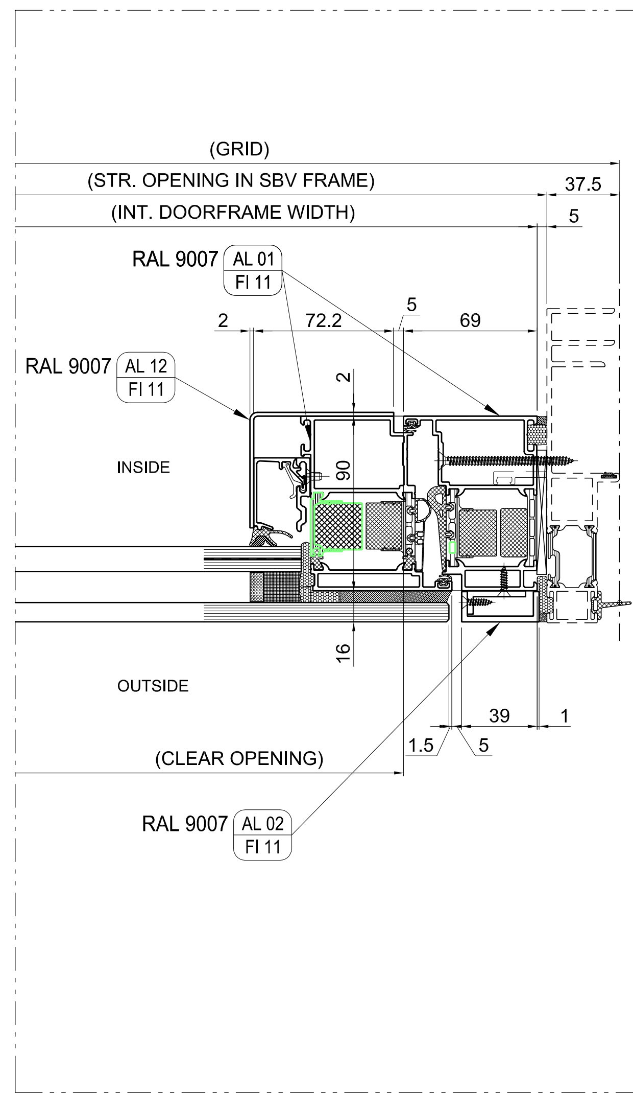
11 HORIZONTAL SECTION Door type 15 Single Scale: 1:2
