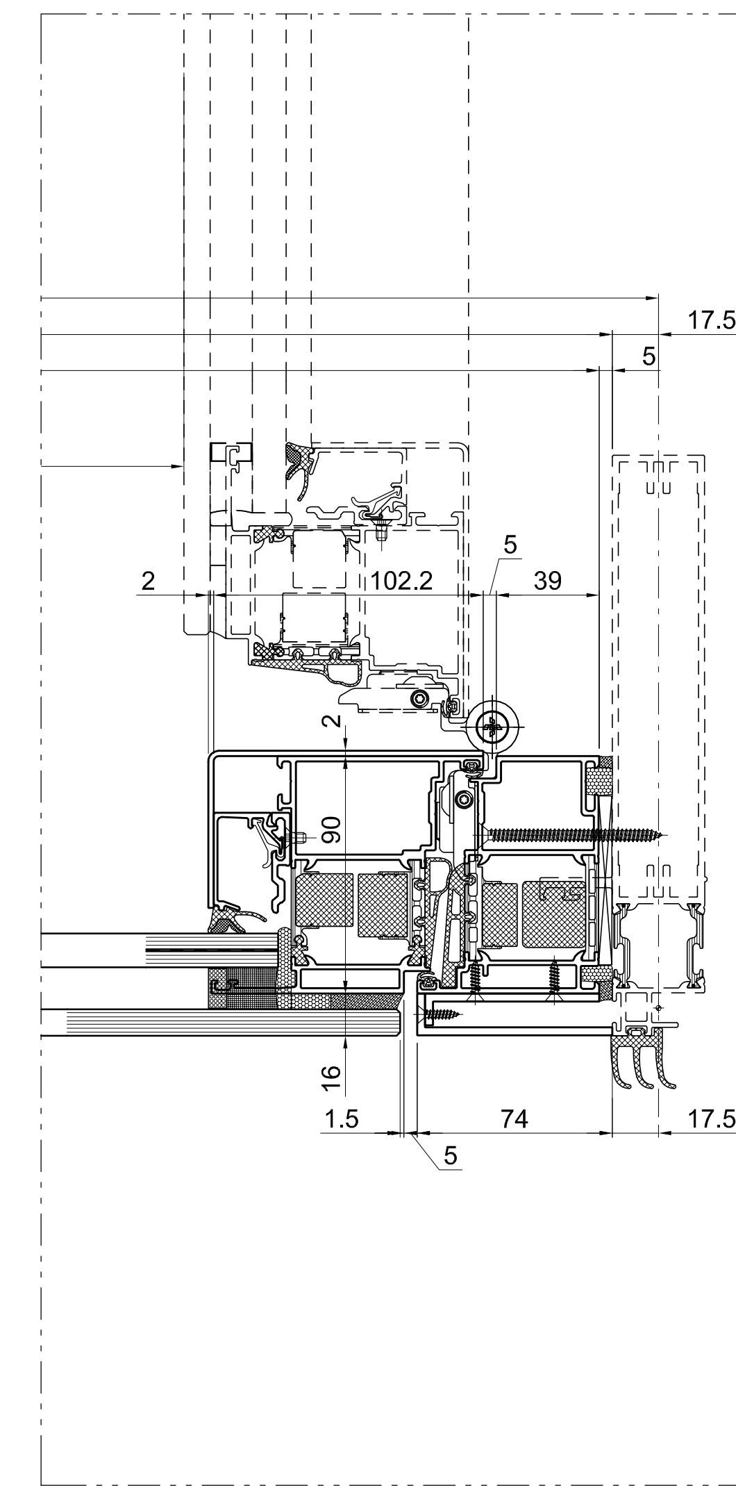
15 HORIZONTAL SECTION Door type 15 Single Scale: 1:2
