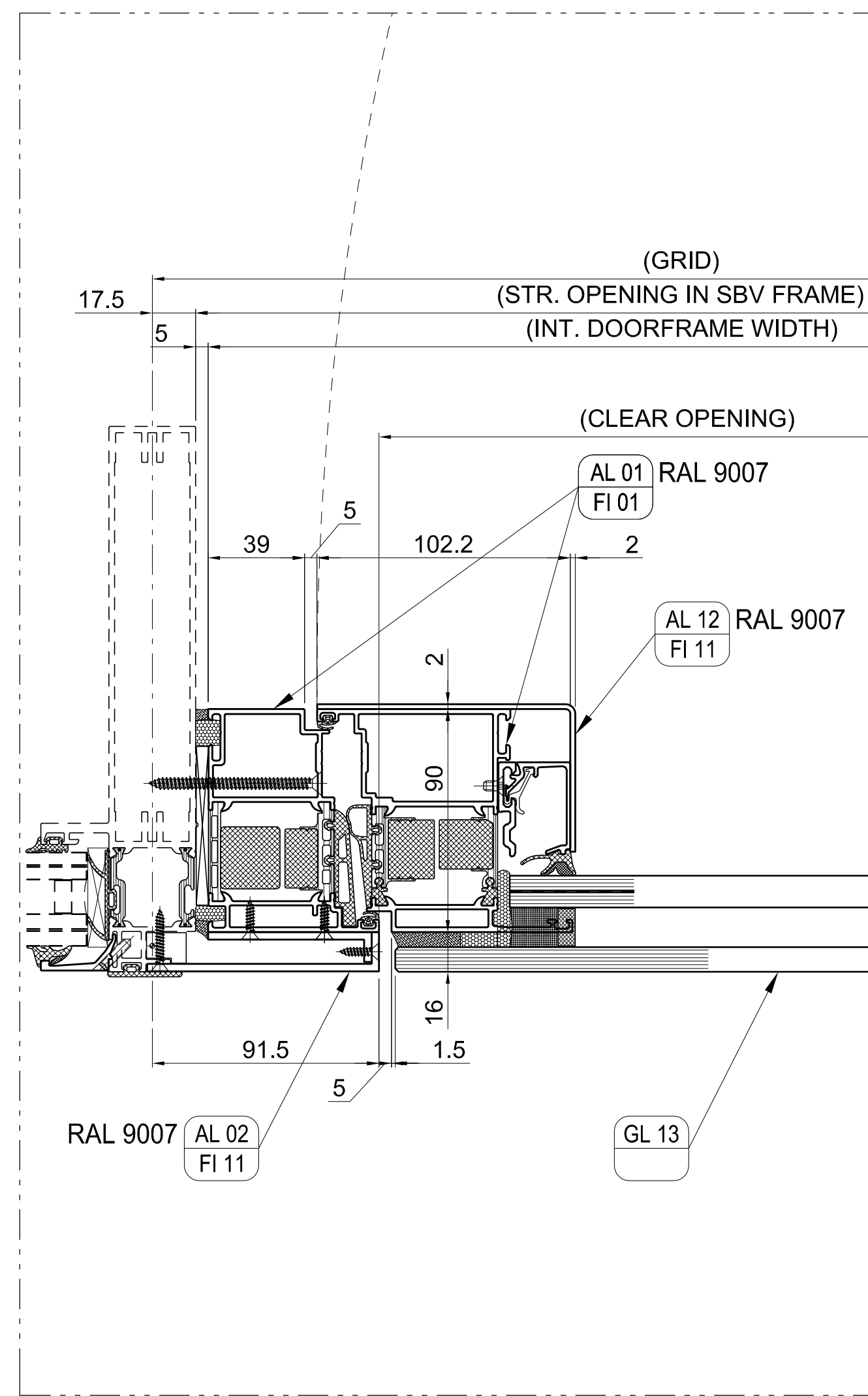
14 HORIZONTAL SECTION Door type 15 Single Scale: 1:2
