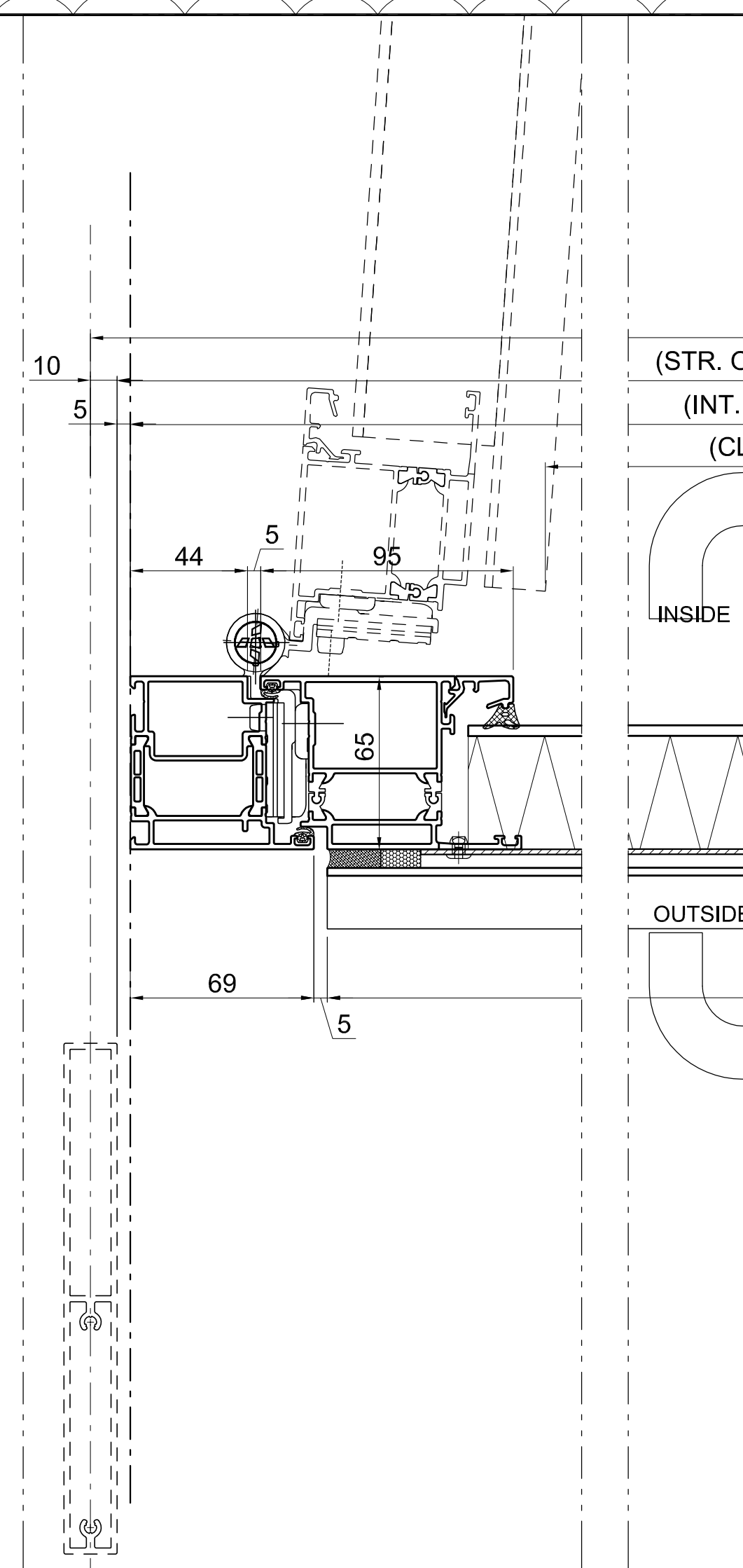
6 HORIZONTAL SECTION Door type 12 Single Scale: 1:2
