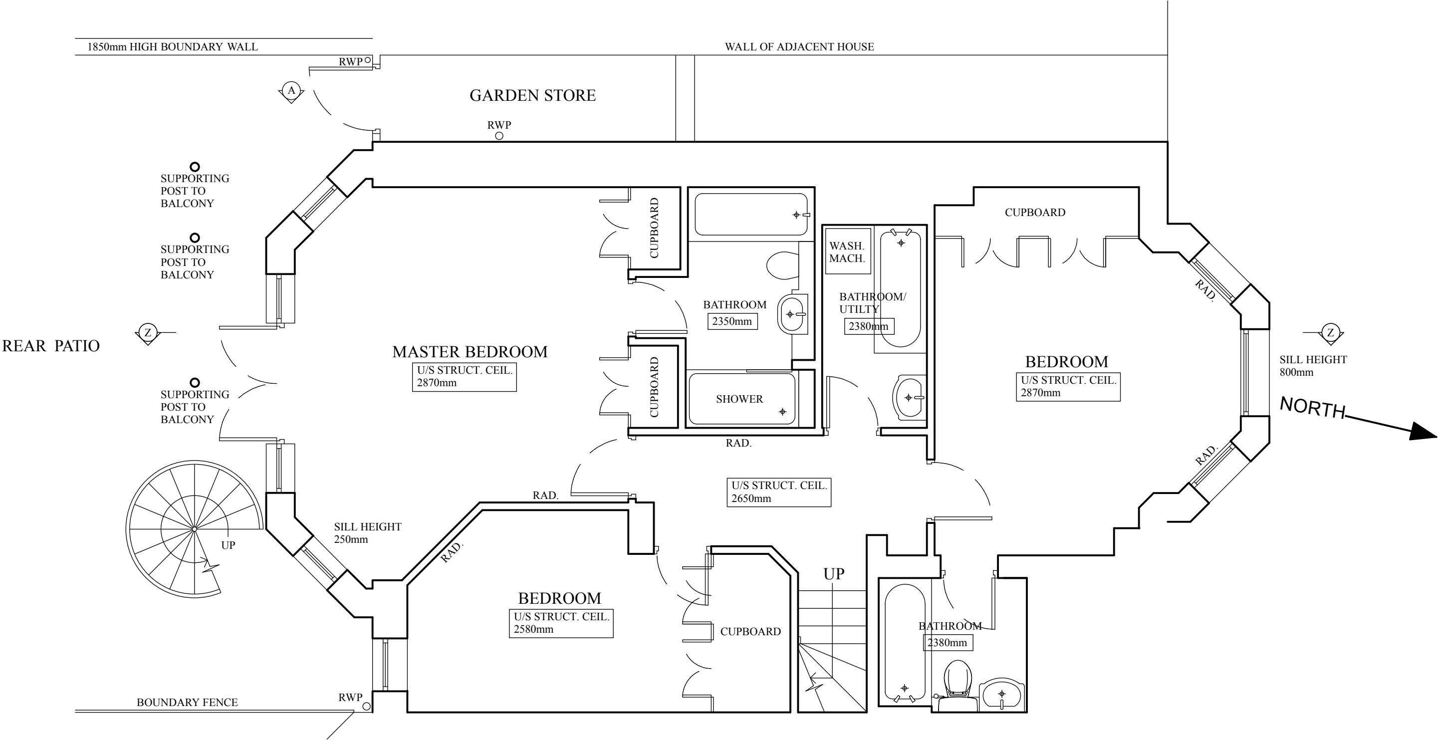
EXISTING LOWER GROUND FLOOR PLAN
