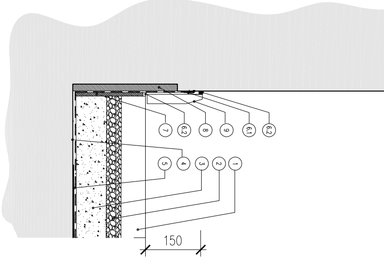
EDGE CONDITION 3* - CONCRETE JUNCTION
