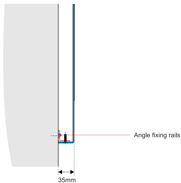
Section through - scale 1:5 @ A3
