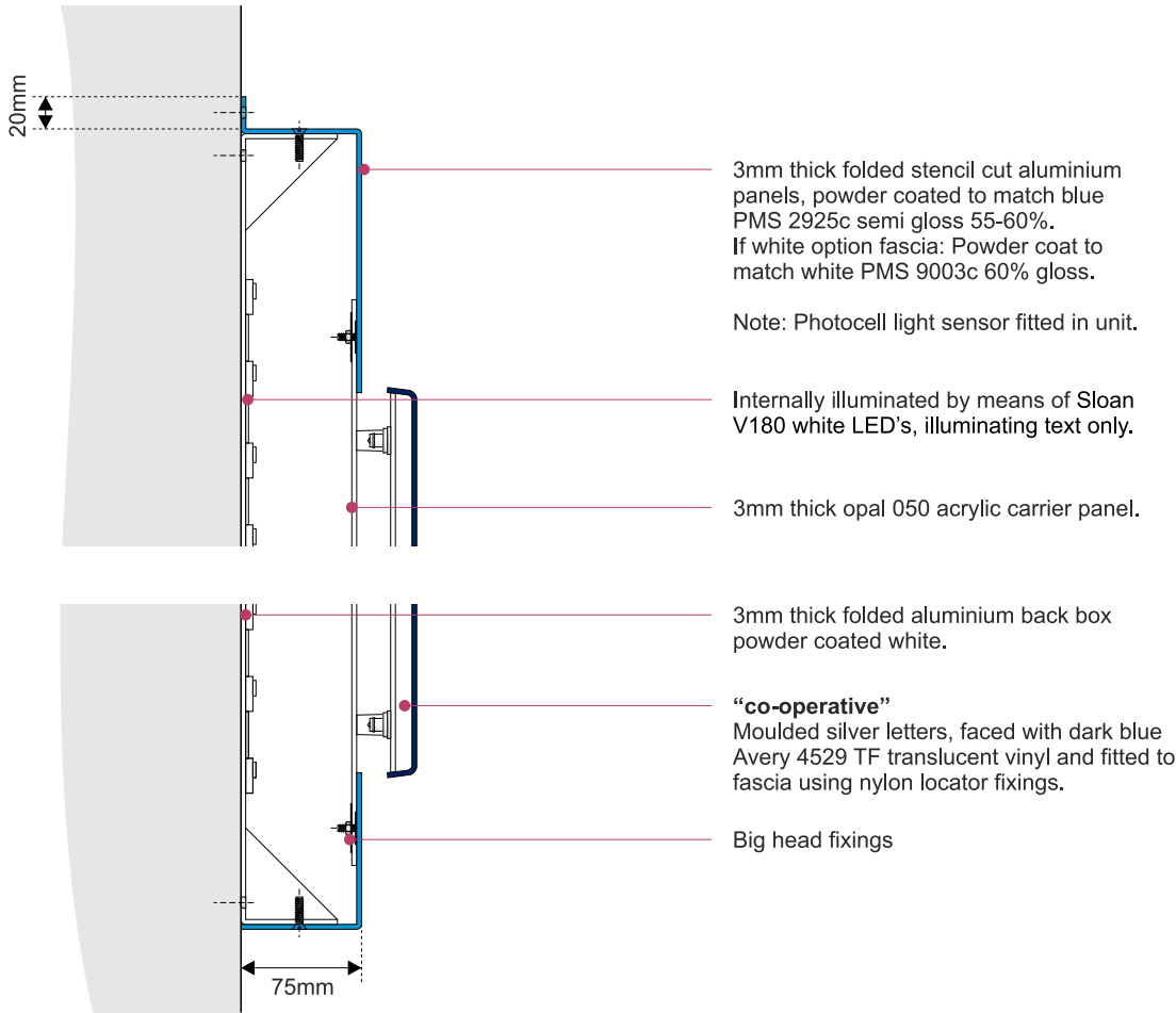
Item 3 - scale 1:20 @ A3 (M3 Lettering)
