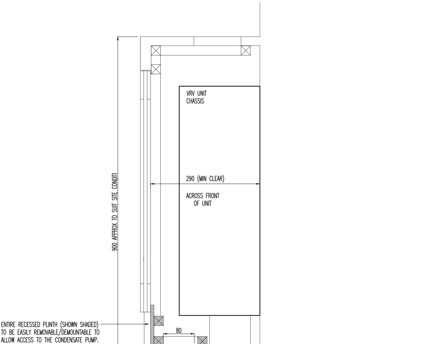
SIDE VIEW
