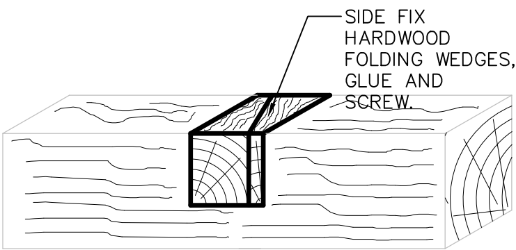
NOTCH REPAIR DETAIL 2 FOR NOTCHES GREATER THAN 25mm DEEP.
