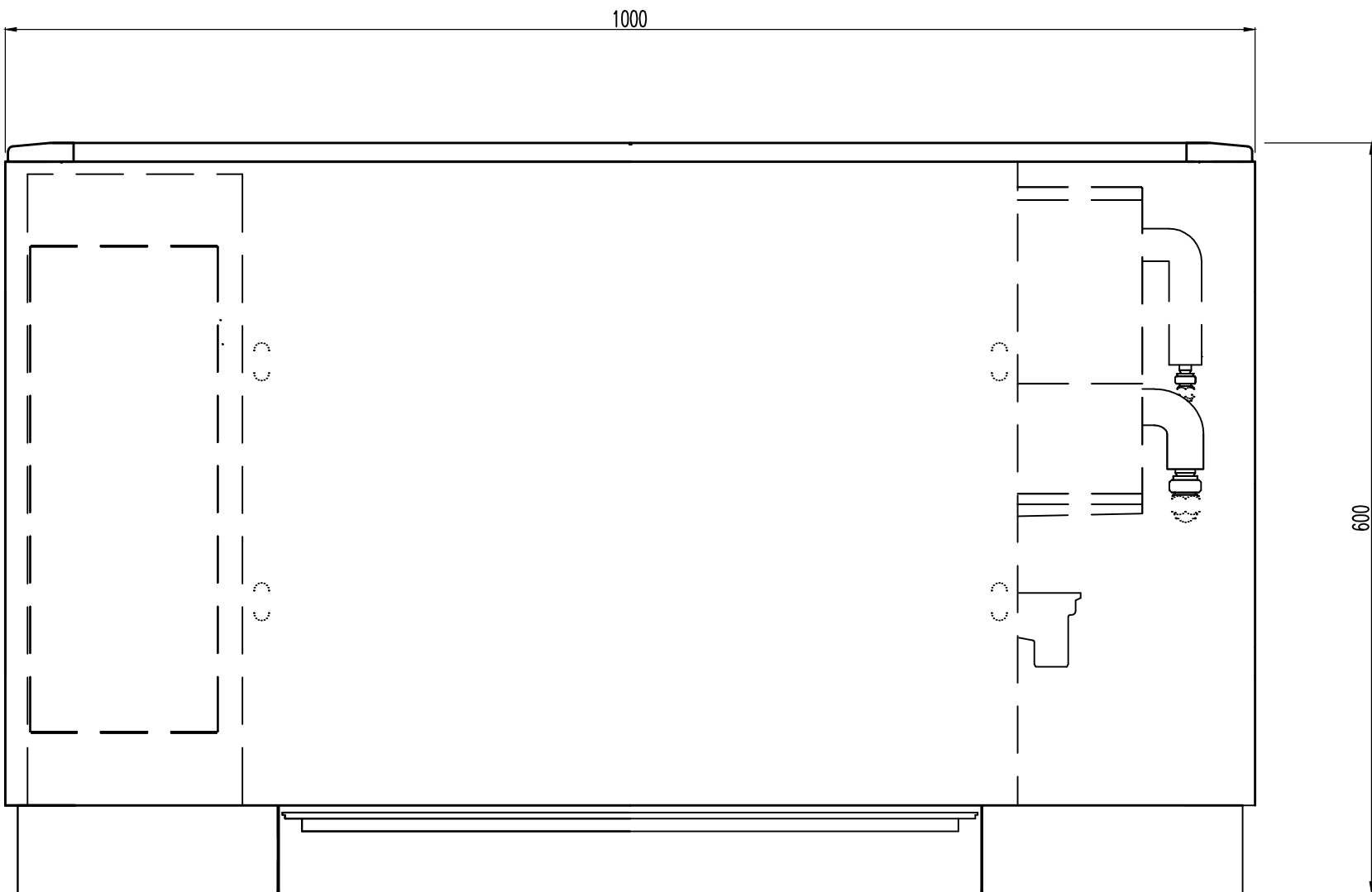
FRONT VIEW
