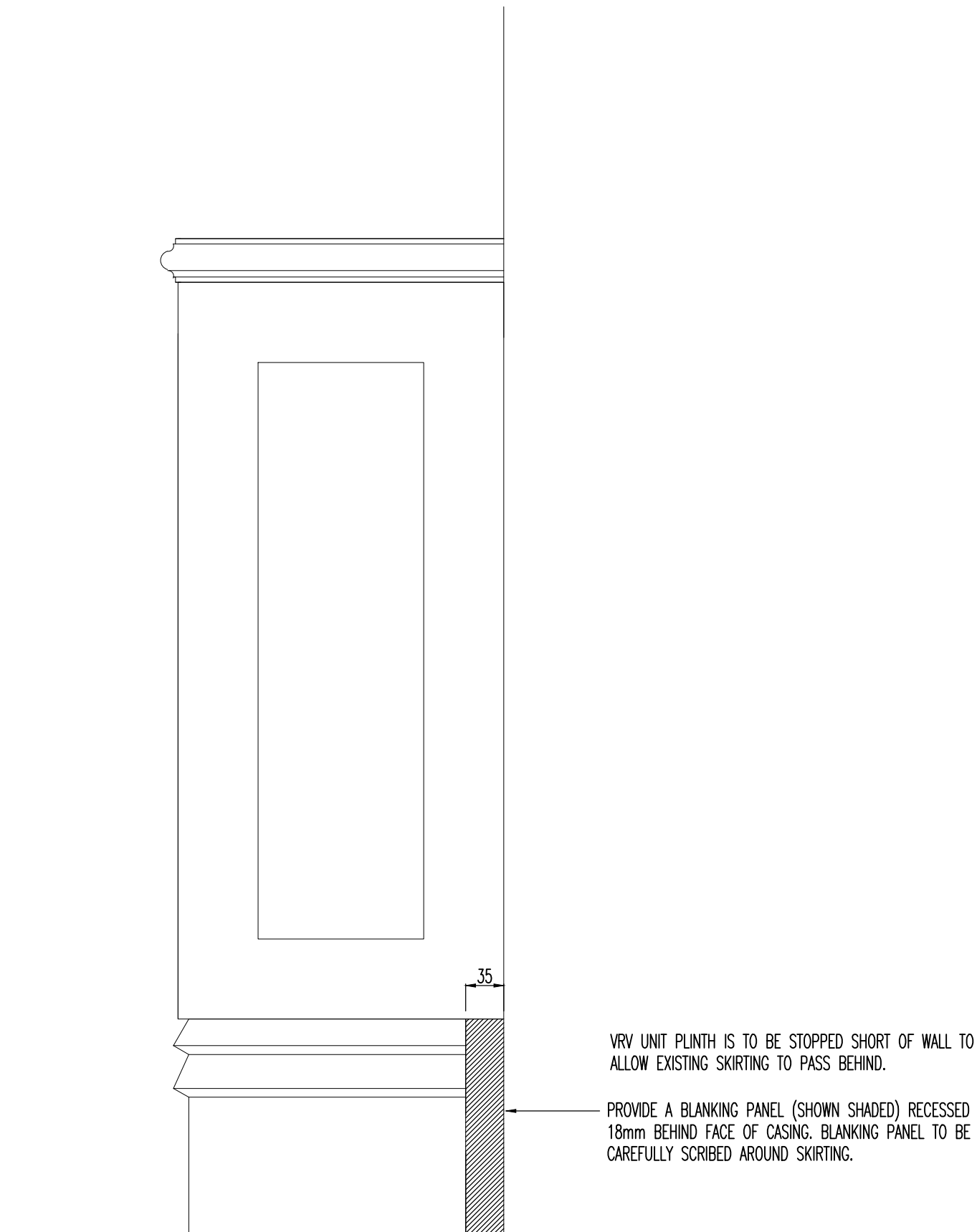
SIDE VIEW
