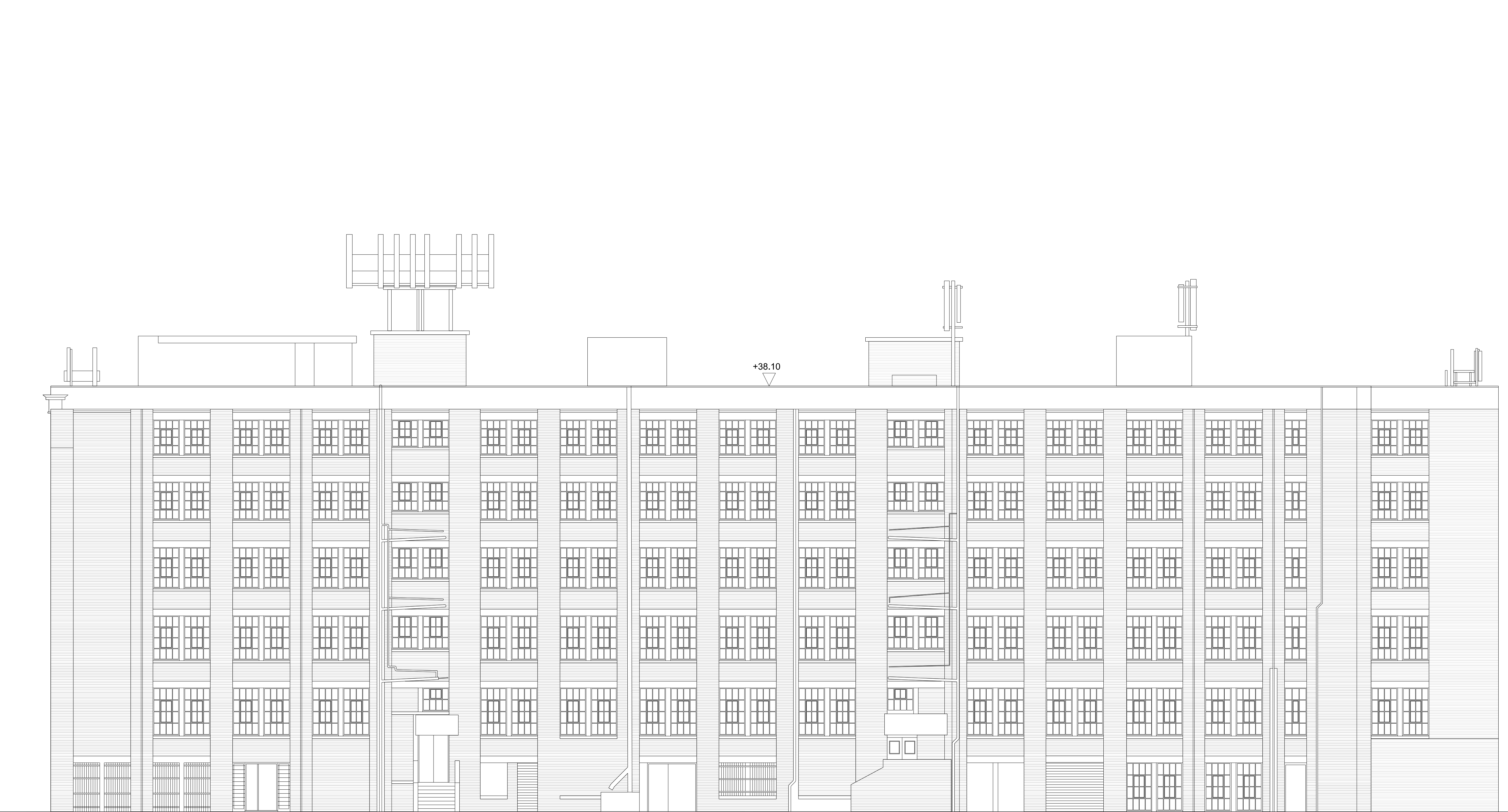
1 West elevation as existing 152_032 Scale 1:100 @ A1
