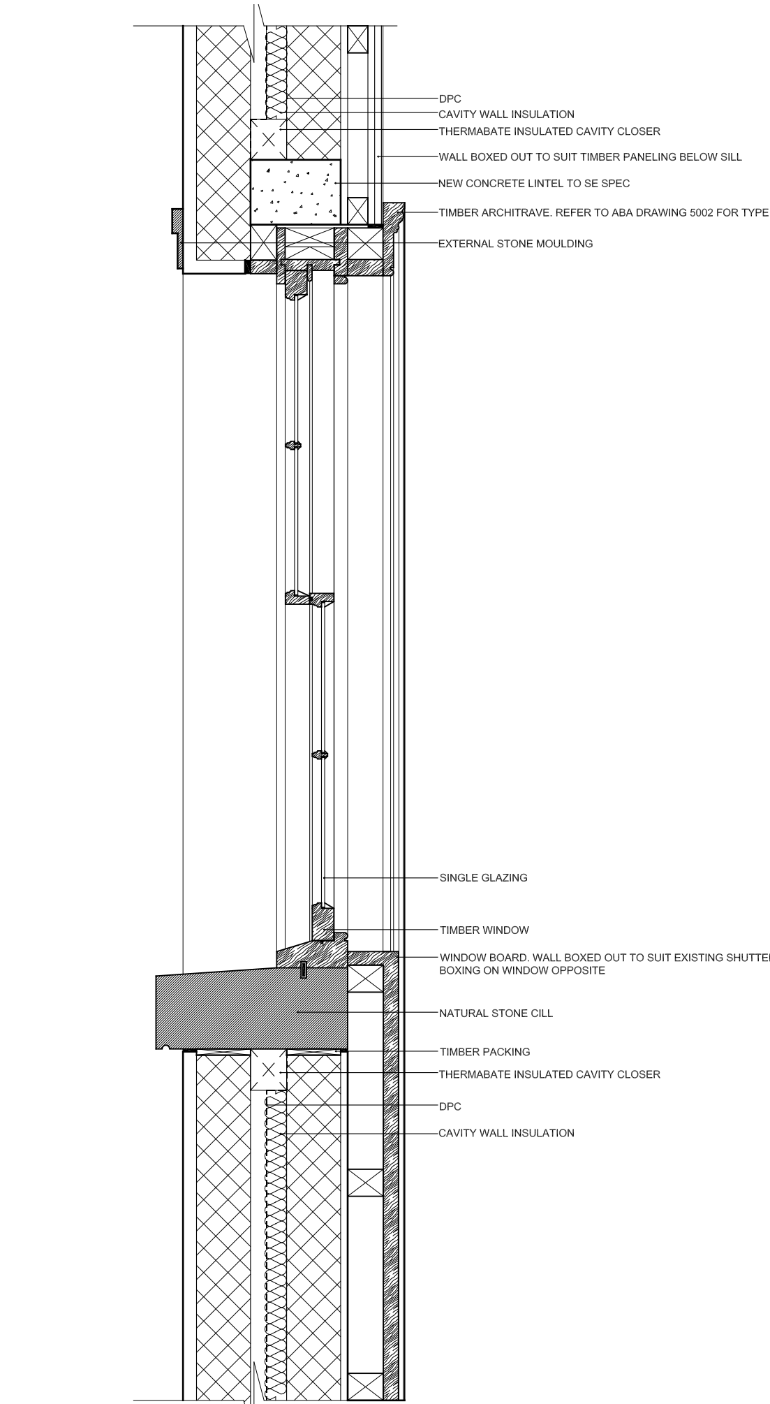
01 TYPICAL WINDOW VERTICAL SECTION 1:10 @ A3
