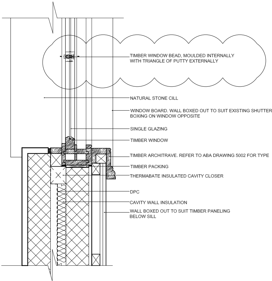
02 TYPICAL WINDOW HORIZONTAL SECTION 1:10 @ A3
