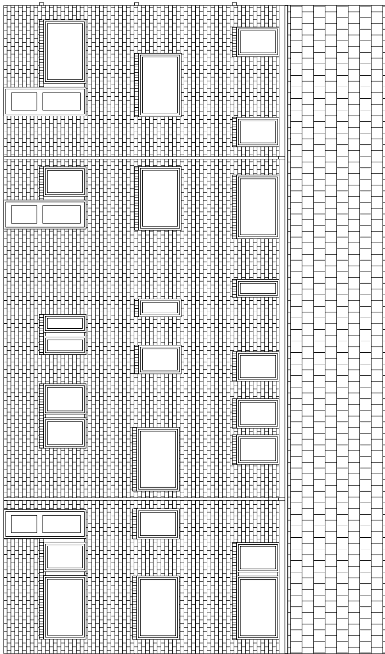
35 - 39 BEAUMONT WALK EXISTING ELEVATION B
