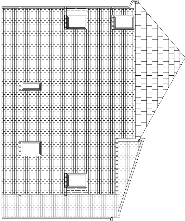
35 - 39 BEAUMONT WALK EXISTING ELEVATION A
