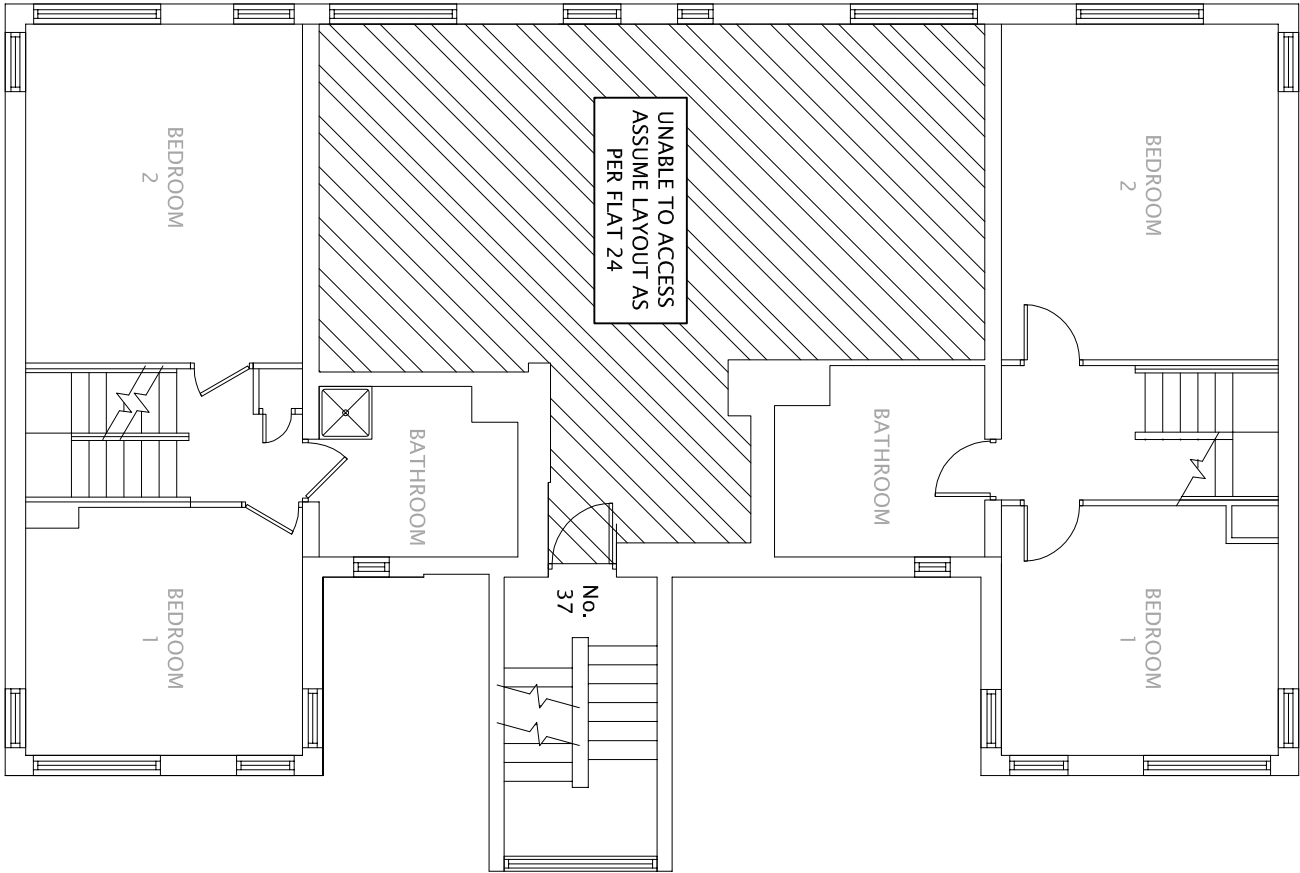
35 - 39 BEAUMONT WALK EXISTING FIRST FLOOR
