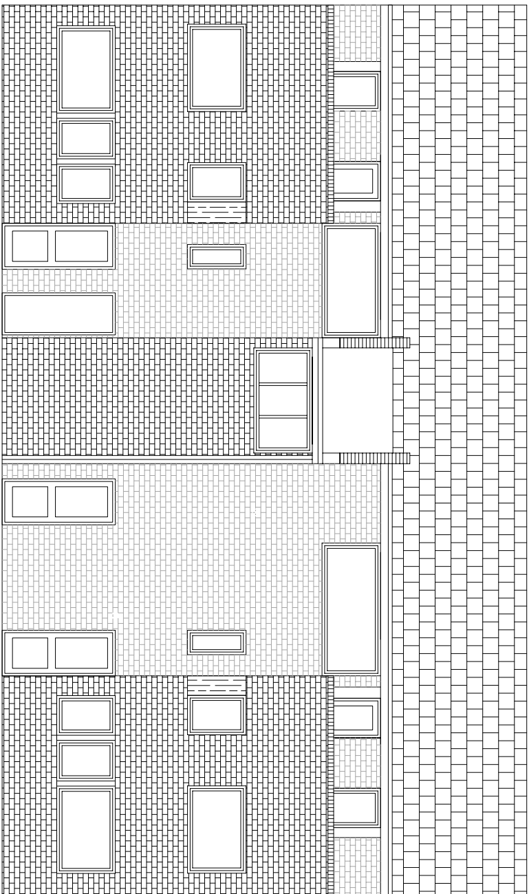
35 - 39 BEAUMONT WALK EXISTING ELEVATION D
