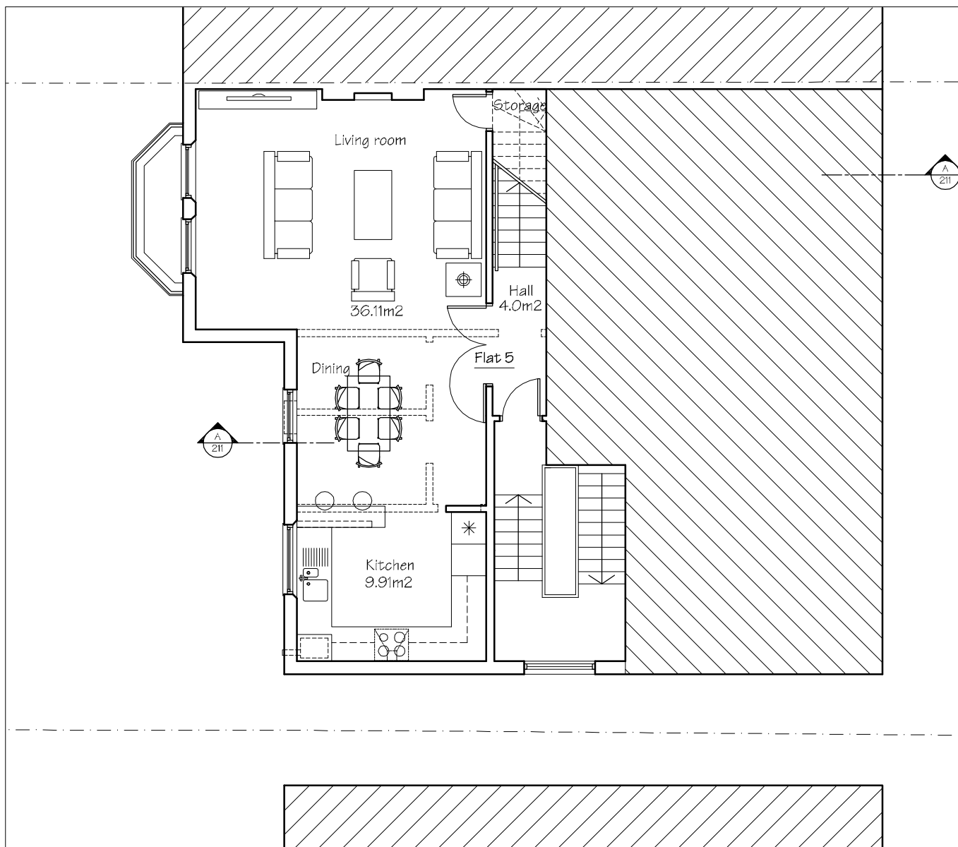
Second Floor Plan as Approved and Proposed - Flat 5
