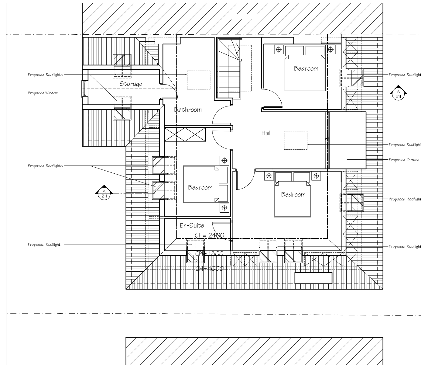
Third Floor Plan as Proposed - Flat 5
