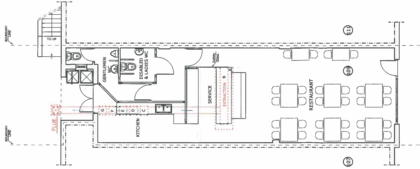
GROUND FLOOR PLAN SCALE: 1/100
