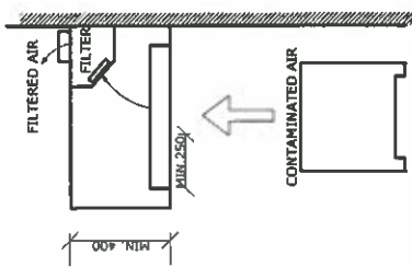
OVERHEAD WALL MOUNTED CANOPY
