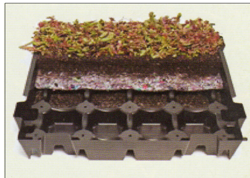
Modular Sedum Pod with Small Pods on a Drainage Tray
