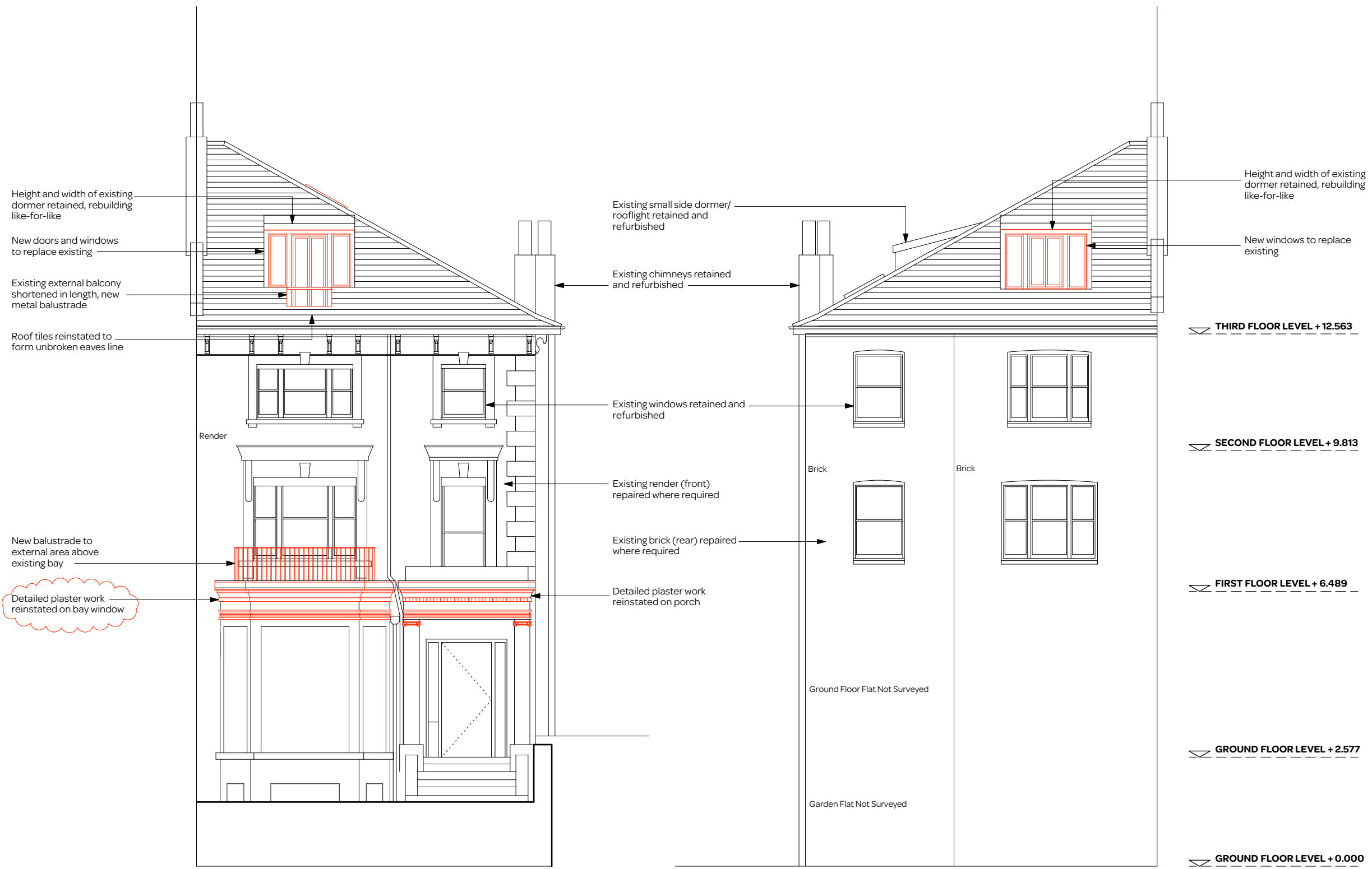
Front Elevation (Part Surveyed)
