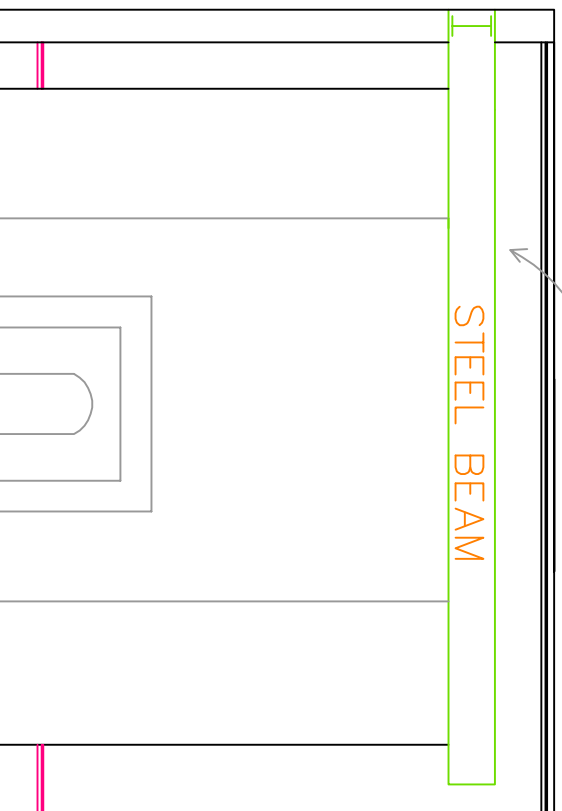
Barrister Room 3 view towards Barrister Room 2 PROPOSED SECTION THROUGH B-B
