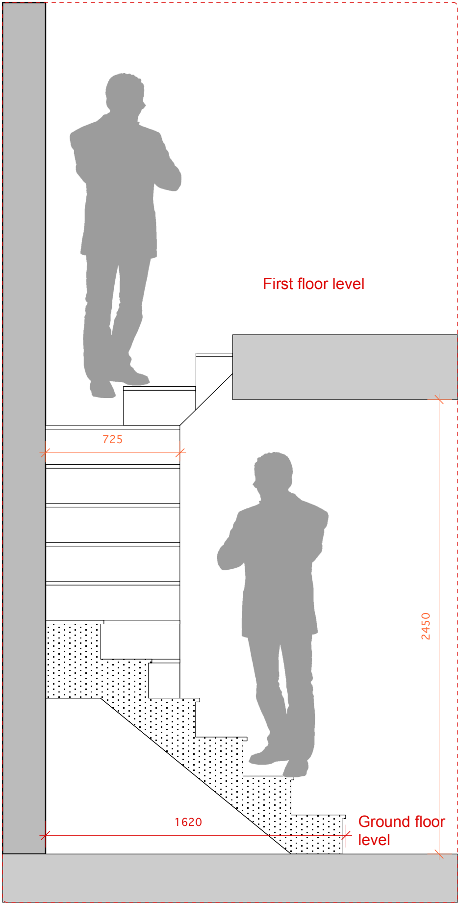
Section AA Staircase Escale: 1:20@A3
