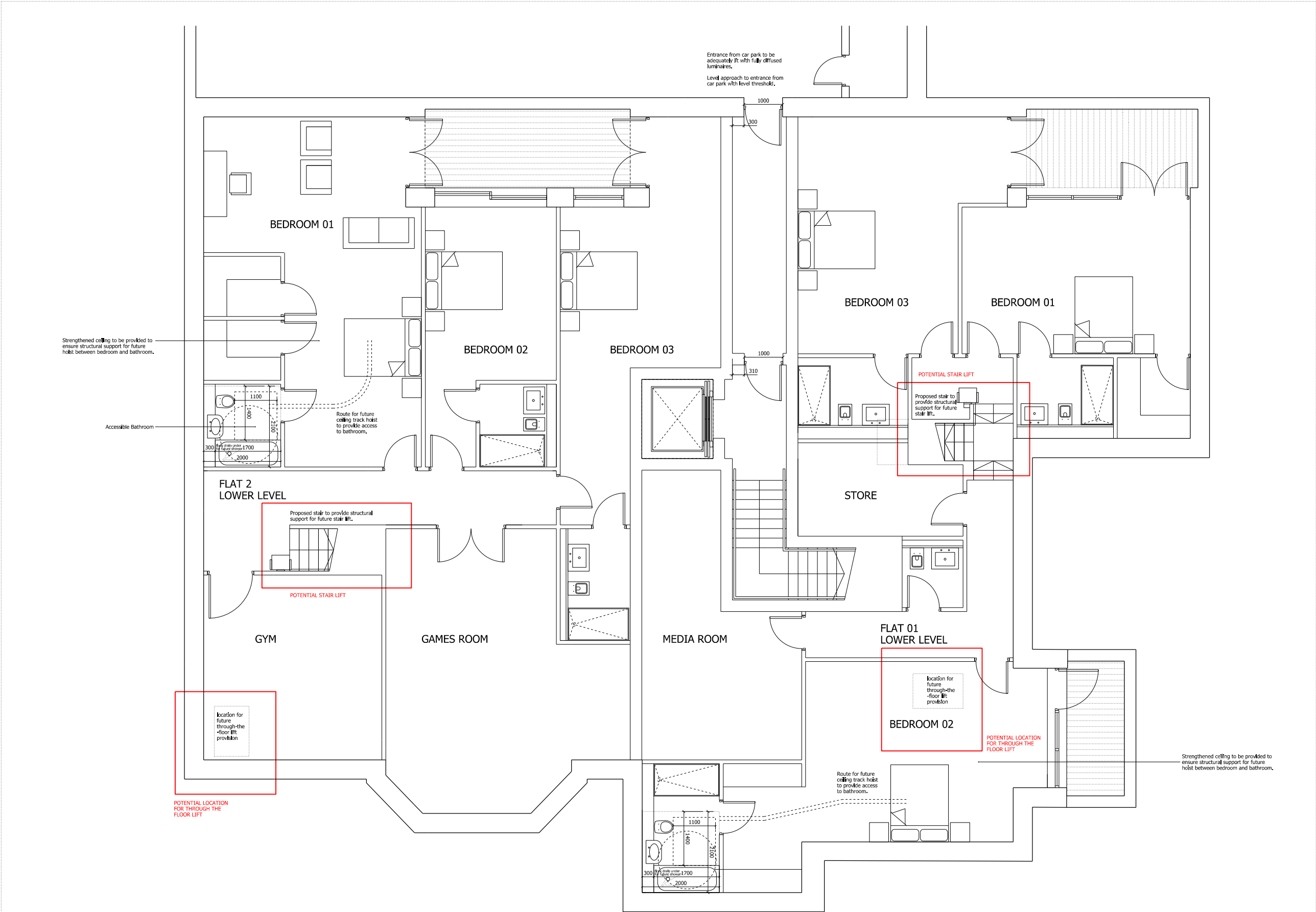
INTERNAL LAYOUT PLAN FLAT 2, LEVEL B1
