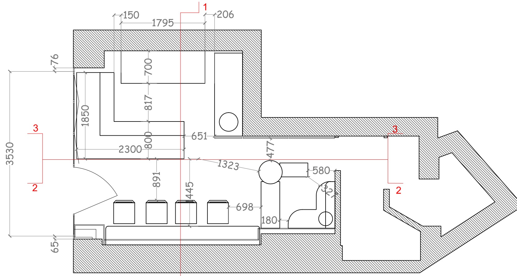
General Arrangement Plan 1
