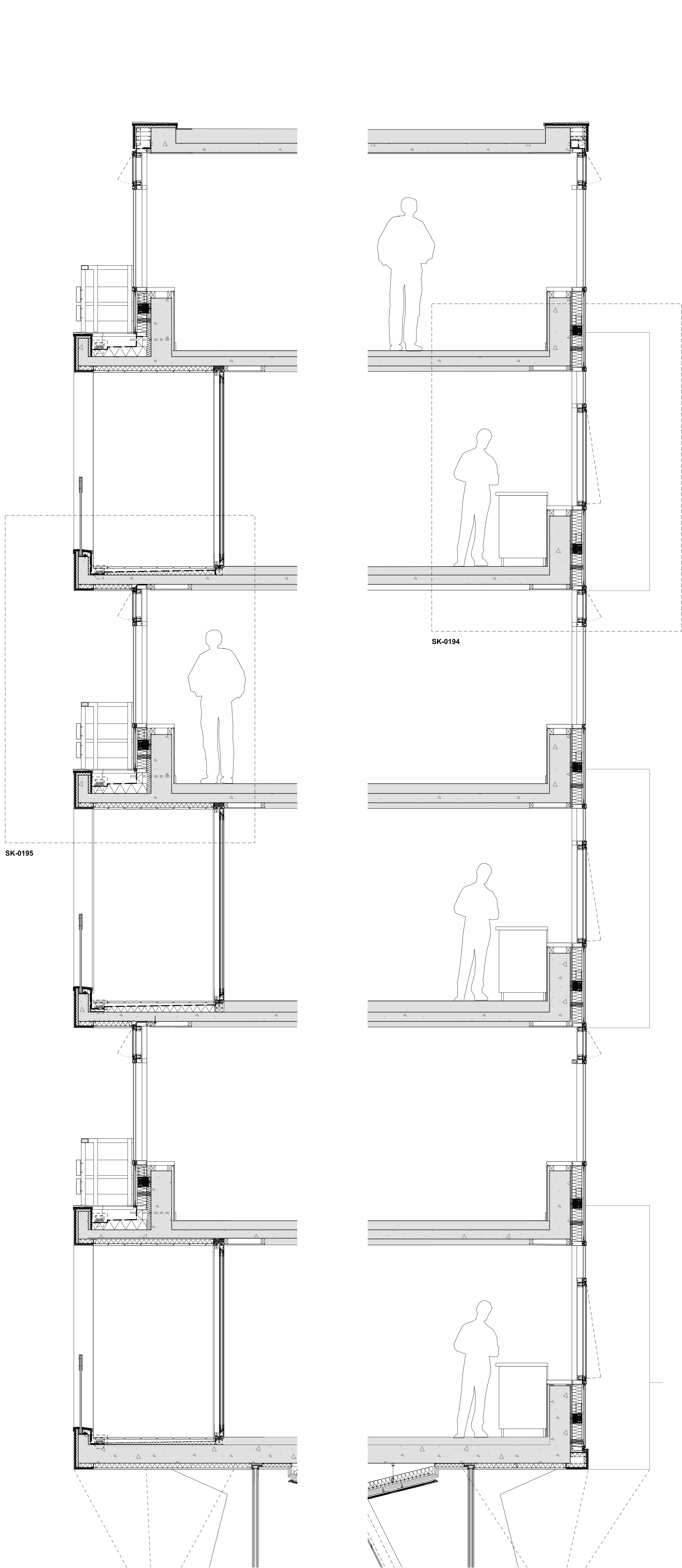
Proposed Section A
