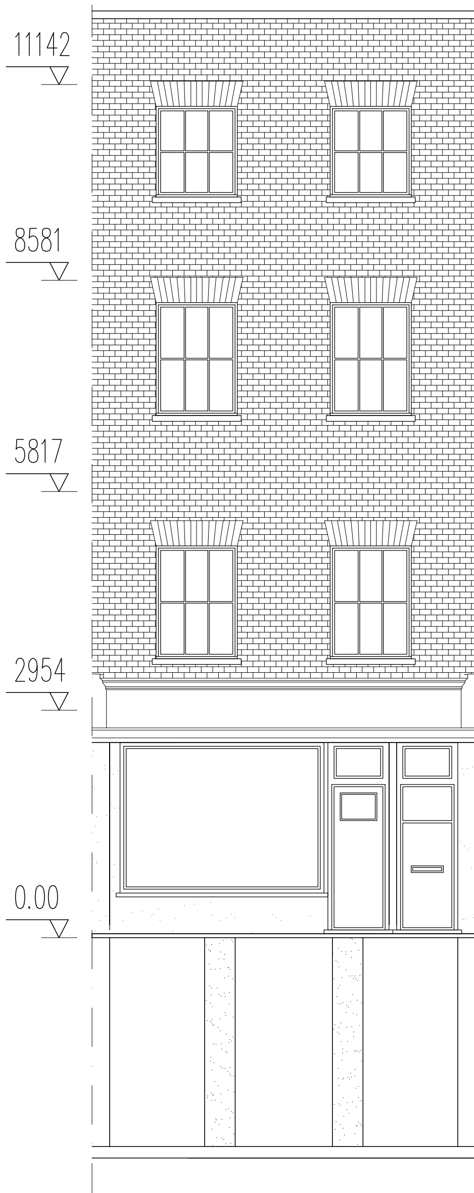
Front Elevation as Existing Showing Lightwell
