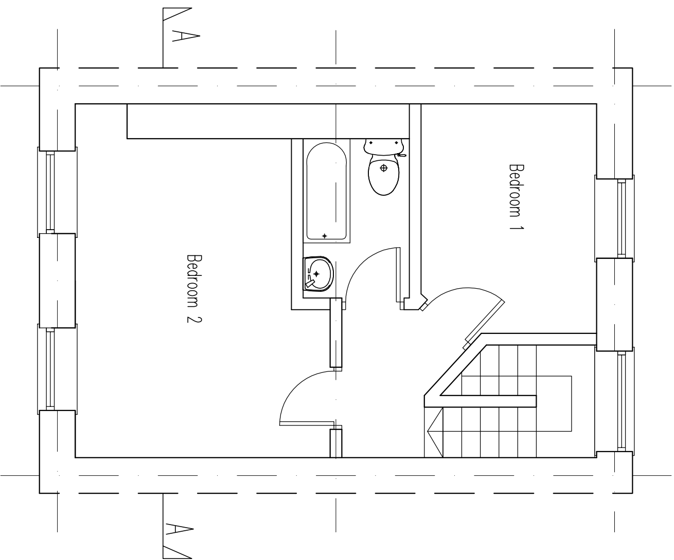
Third floor Plan as Existing
