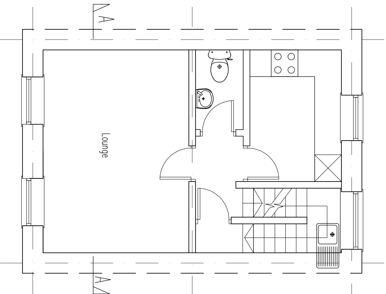
Second floor Plan as Existing
