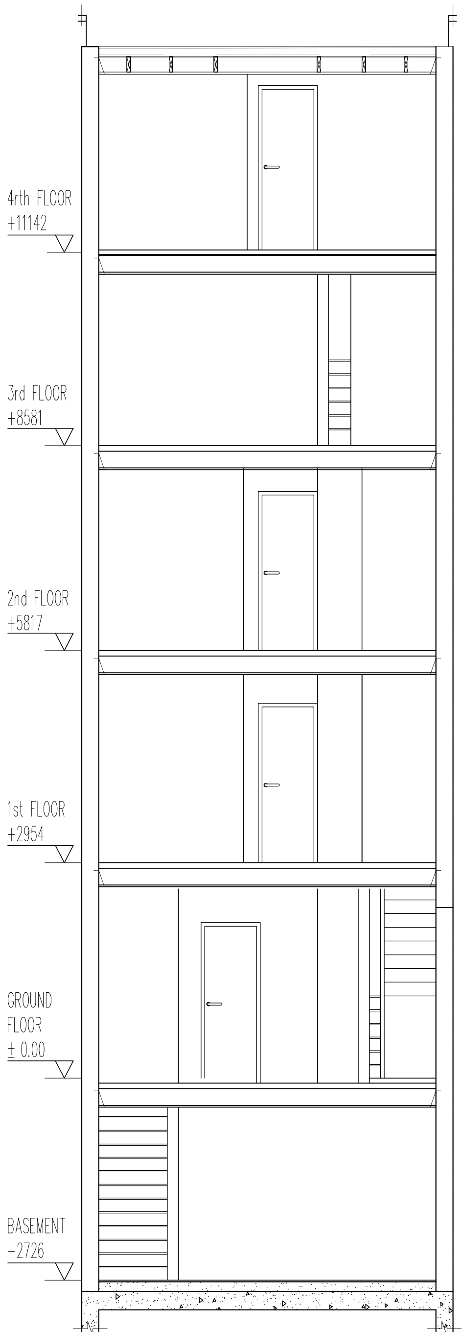
Section AA as Proposed
