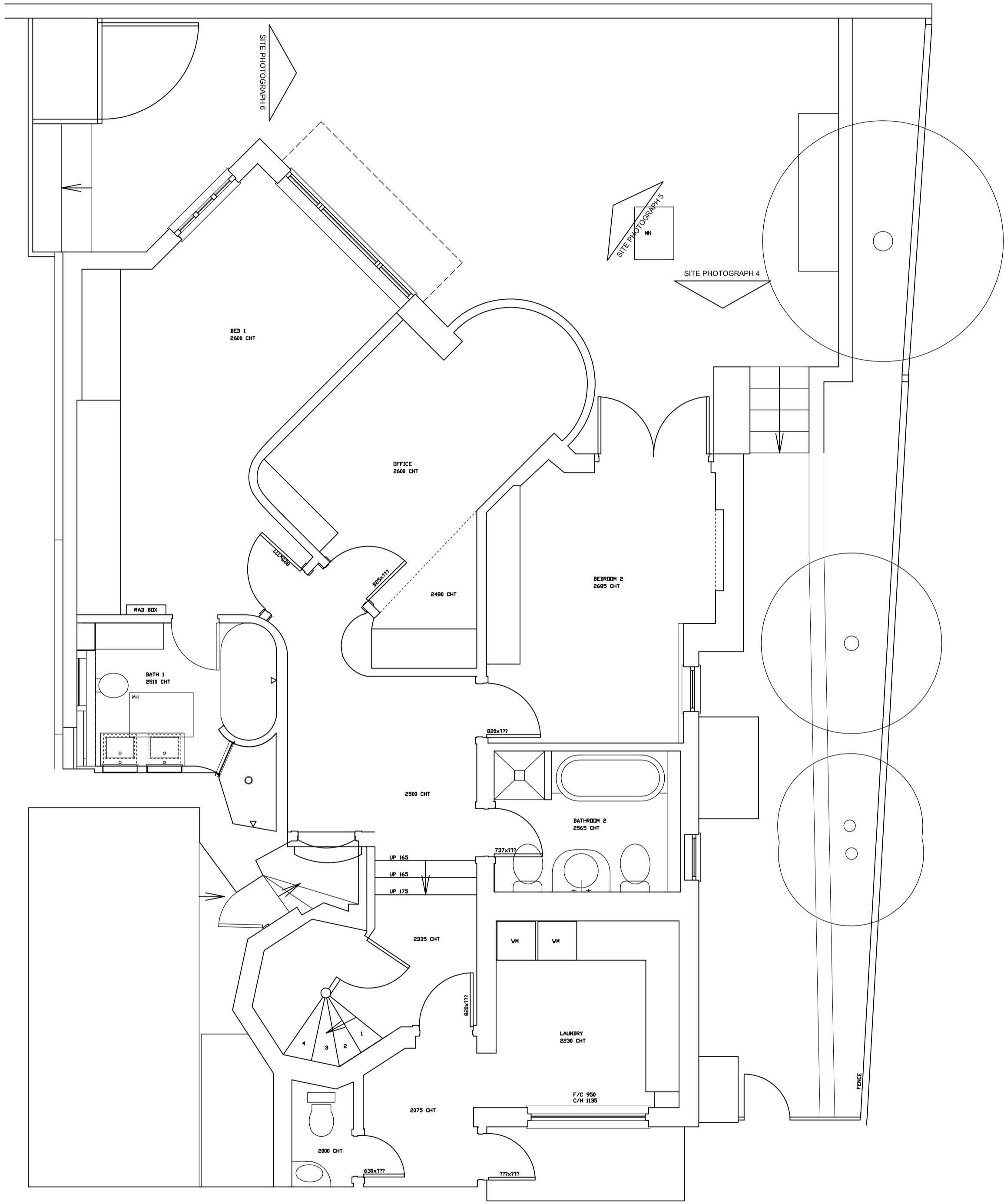
BASEMENT PLAN
