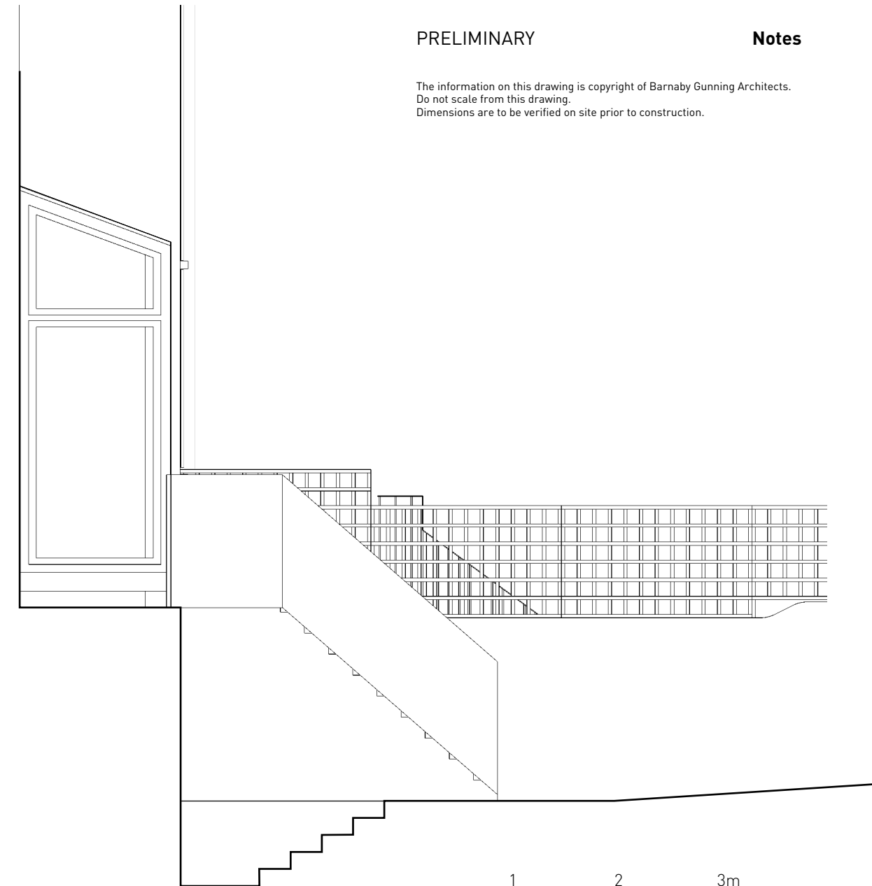
Side Elevation to 25 Gayton Road
